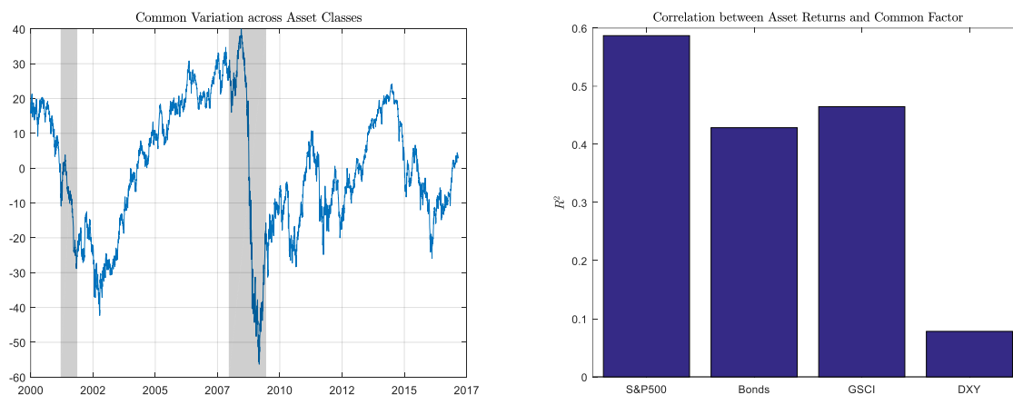
Figure 8. Left: Common variation across asset classes with shaded areas representing NBER-dated recessions. Right: R^2 from projecting individual asset returns on the common factor
