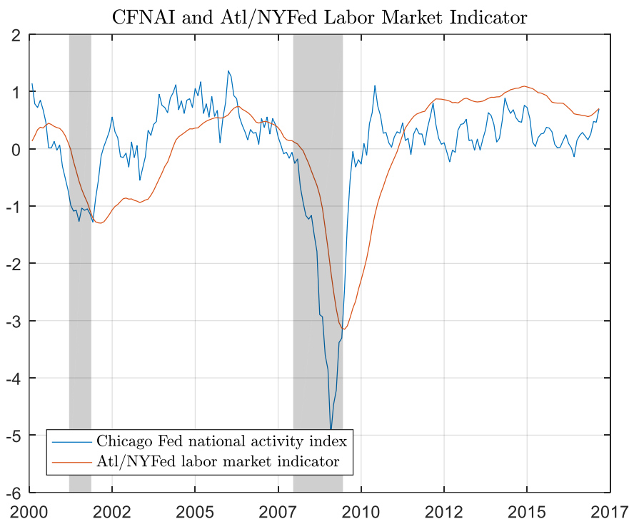
Figure 10. Chicago Fed national activity index (CFNAI) and Atlanta Fed and New York Fed (AtlFed/NYFed) labor market indicator. Shaded areas are NBER-dated recessions
