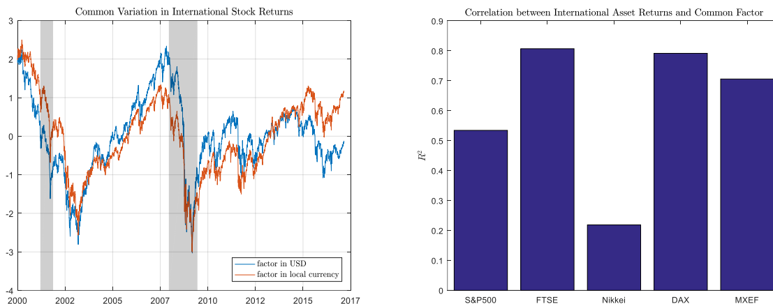
Figure 9. Left: Common variation in international stock returns with shaded areas representing NBER-dated recessions. Right: R^2 from projecting individual stock returns on the common factor
