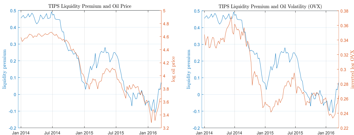
Figure 2. Time plot of weekly TIPS liquidity premium with oil prices and oil option-implied (OVX) volatility
