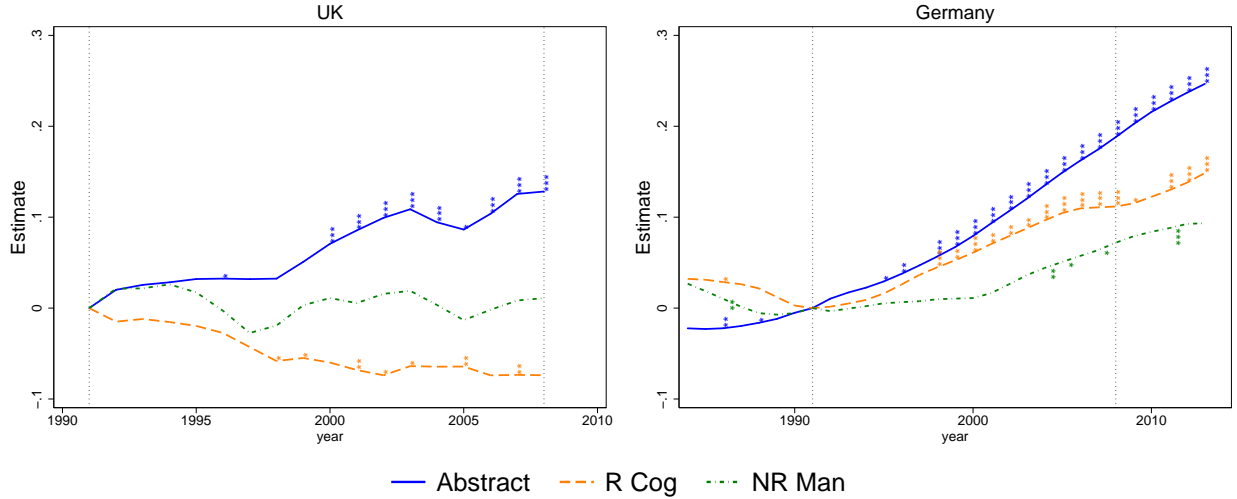
Figure 5: Task Prices Relative to Routine Manual
