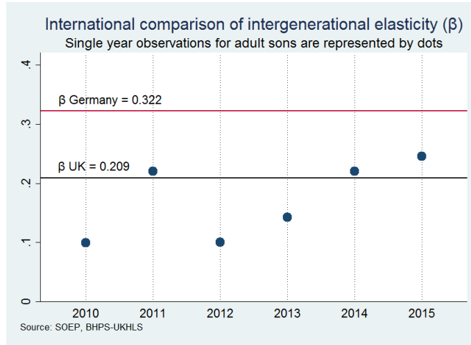
Fig. 3: International comparison of intergenerational elasticity ( \beta )
