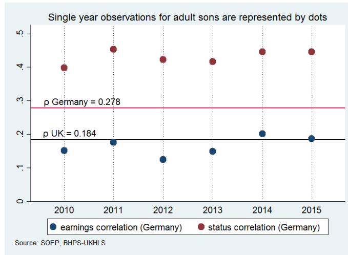
Fig. 4: International comparison of intergenerational correlation ( \rho )
