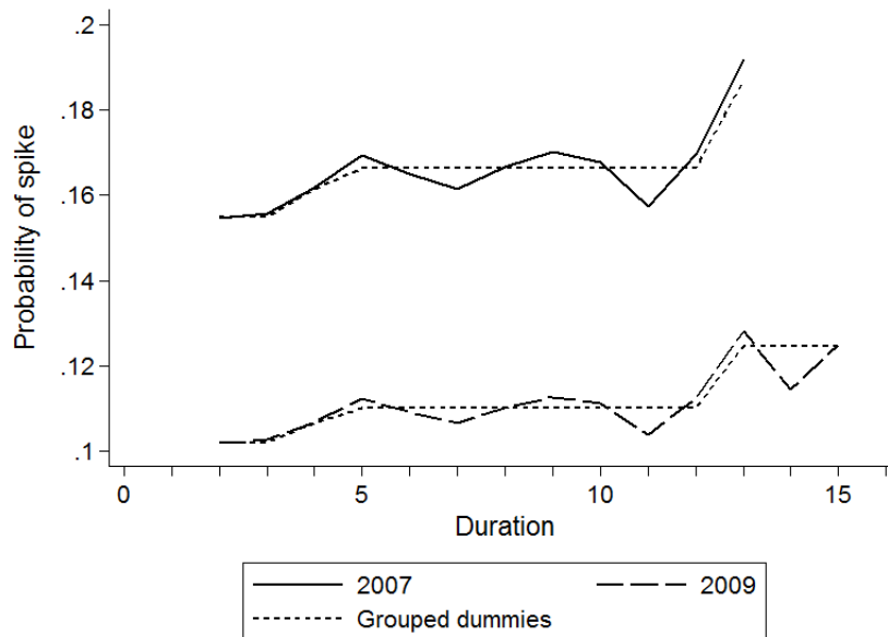
Figure 3.1: Baseline hazard
