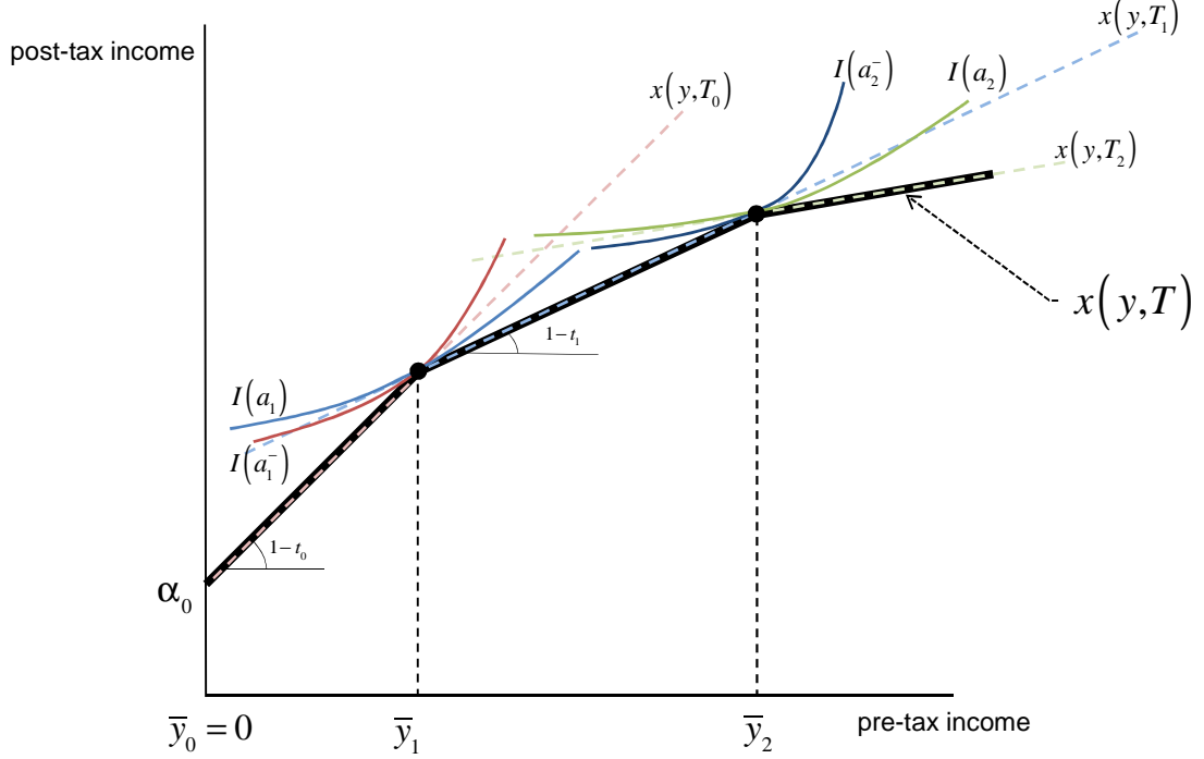
Figure 3: Figure for Theorem 2
