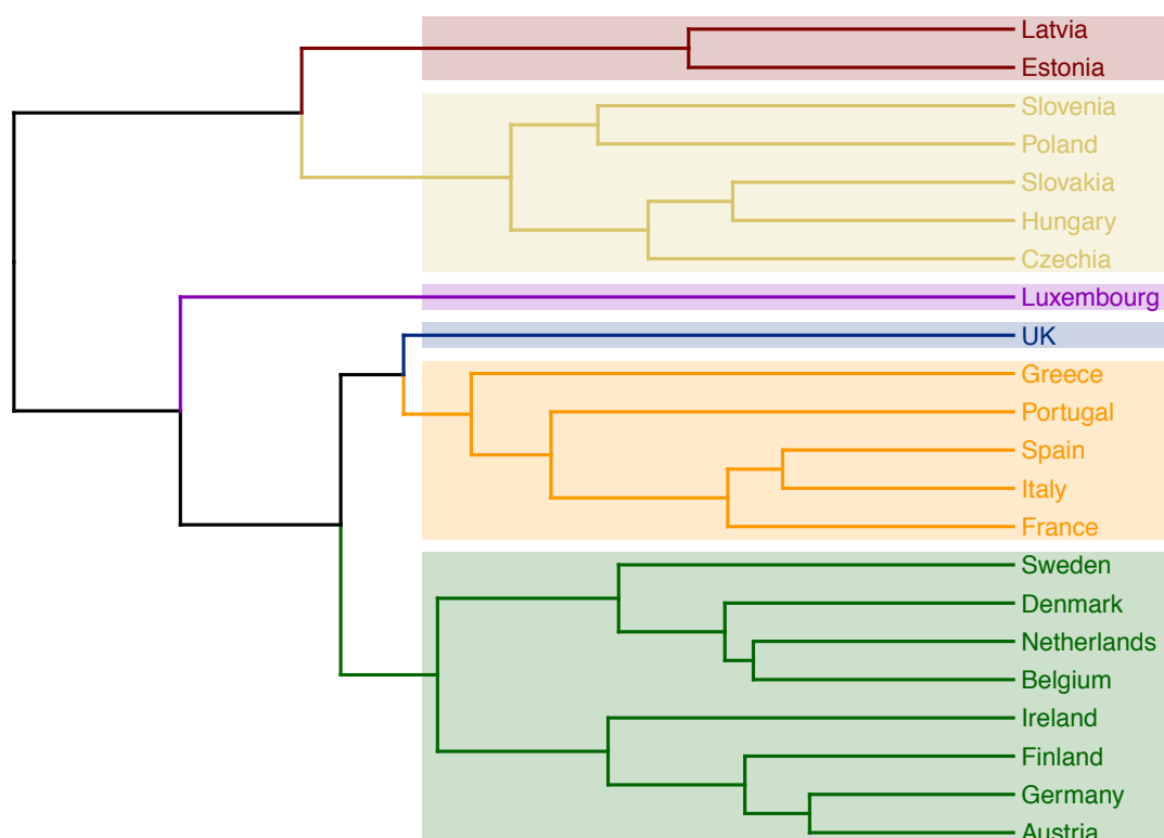
Cluster Dendrogram
