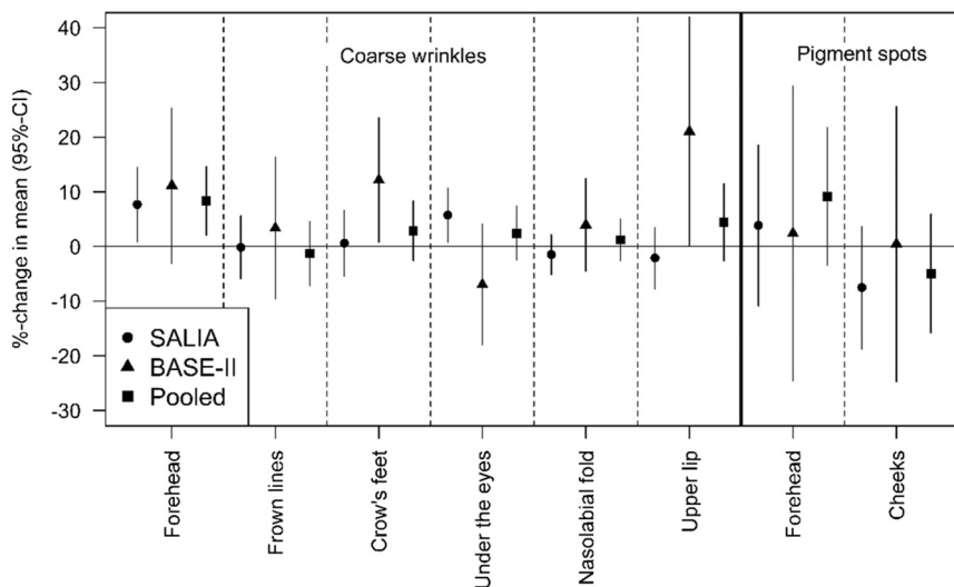
Fig. 1. Title: O 3 exceedance days [7 days/year] with scores for extrinsic skin aging in the study cohorts.
