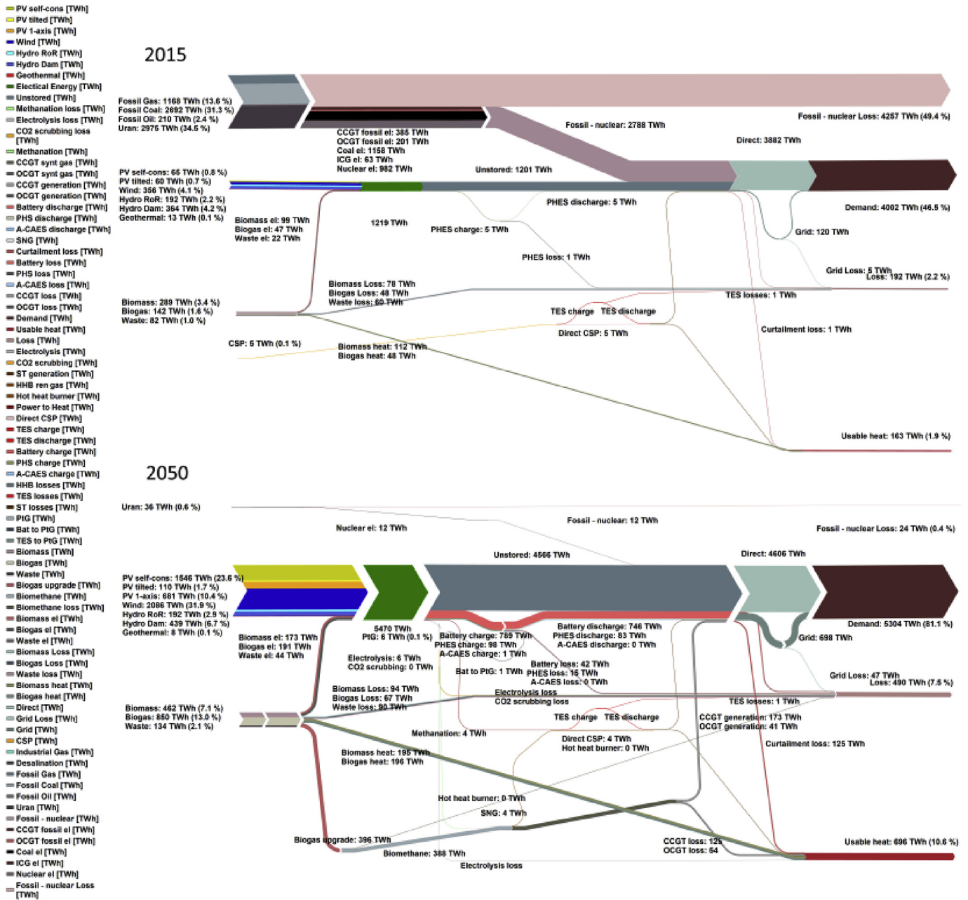
Fig. 19. Energy flow diagrams for the Area scenario in 2015 (upper) and 2050 (lower).
