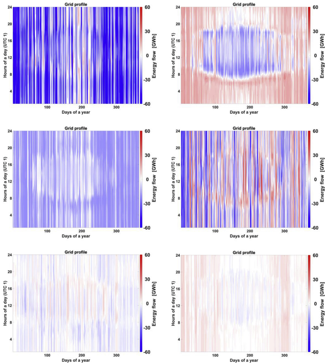
Fig. 16. Example profiles of six different types of grid use for net exporters of wind energy (BRI - upper left), net exporters of solar PV energy (IT - upper right), net exporters of wind and hydropower (NO - middle left), large balancing regions (DE - middle right), small balancing regions (AUH - lower left), and net importers (CH - lower right).
