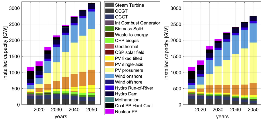
Fig. 8. Installed generation capacities from 2015 to 2050 for the Regions (left) and Area (right) scenarios. Adapted from Ref. [39].
