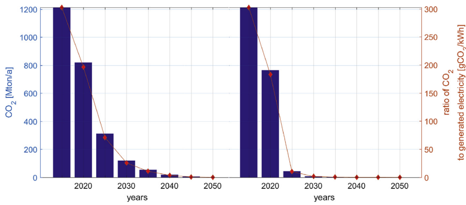
Fig. 21. GHG emissions in the Regions (left) and Area (right) scenarios for the period of 2015–2050. Adapted from Ref. [39].
