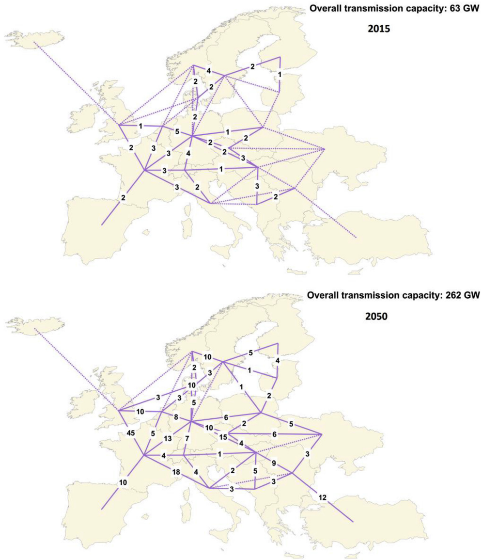
Fig. 12. Interconnection capacity (GW) in the Area scenario for 2015 (upper) and 2050 (lower).
