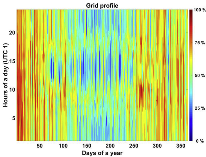
Fig. 14. Grid utilisation profile for the Area scenario in 2050.
