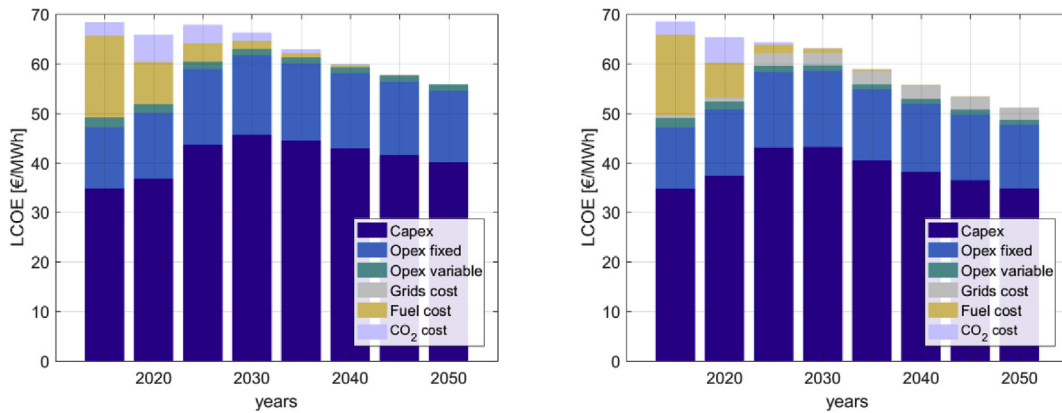
Fig. 22. Levelised cost of electricity and breakdown in cost categories for the Regions (left) and Area (right) scenarios. Grid costs are not accounted for the Regions scenario, as there were no assumed transmission interconnections with neighbouring countries in this scenario.
