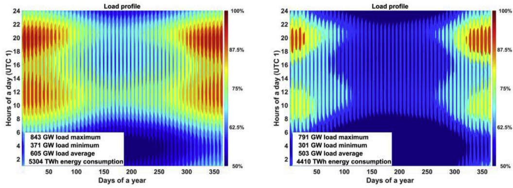
Fig. 20. Load profile of central grid without (left) and with (right) consideration of the impacts of prosumer self-consumption and storage.
