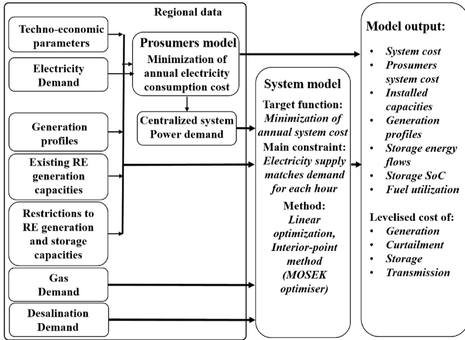
Fig. 5. Main inputs and outputs of the LUT Energy System Transition model. Adapted from Ref. [39].
