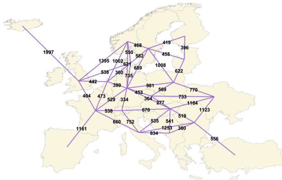
Fig. 7. Interconnections between regions and transmission line lengths (km).
