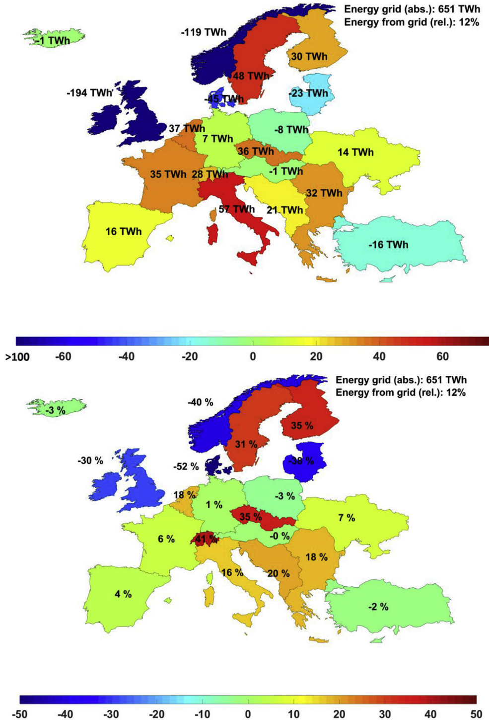
Fig. 17. Absolute annual transmission grid utilisation in TWh (upper) and relative annual grid utilisation as a percent of regional electricity demand (lower) in the Area scenario for the regions of Europe in 2050. Negative values represent net annual export, while positive values represent net annual import. Total grid transmission is 651 TWh, representing 12% of total electricity demand.
