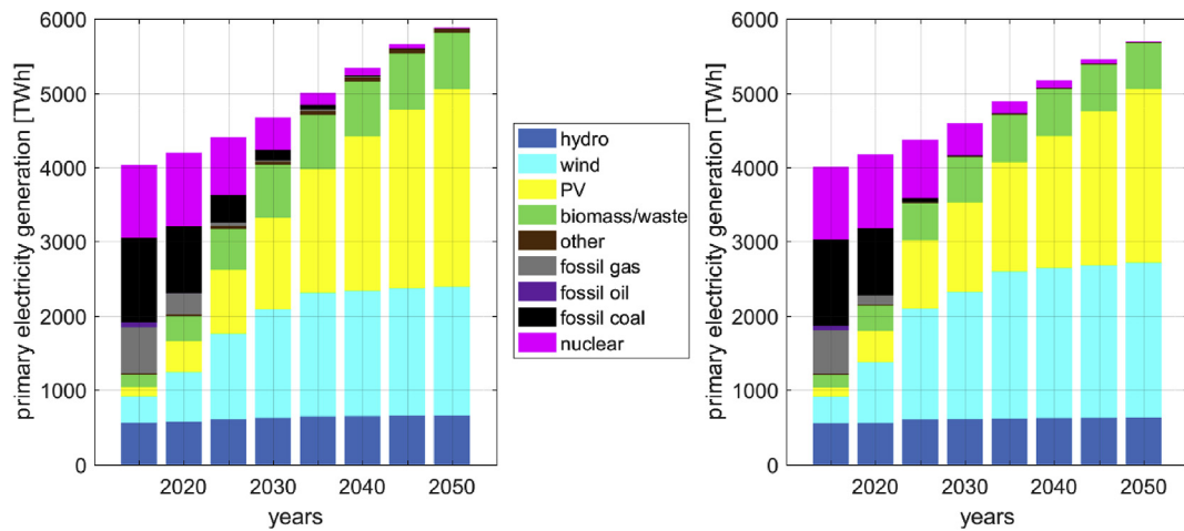
Fig. 9. Electricity generation by fuel from 2015 to 2050 for the Regions (left) and Area (right) scenarios.
