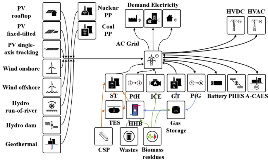
Fig. 6. Block diagram of the LUT Energy System Transition model. Acronyms not introduced elsewhere include: PP - power plant, ST - steam turbine, PtH - power-to-heat, ICE - internal combustion engine, GT - gas turbine, PtG - power-to-gas, PHEs - pumped hydro energy storage, A-CAES - adiabatic compressed air energy storage, TES - thermal energy storage, HHB - hot heat burner, CSP - concentrating solar thermal power. Adapted from Ref. [39].
