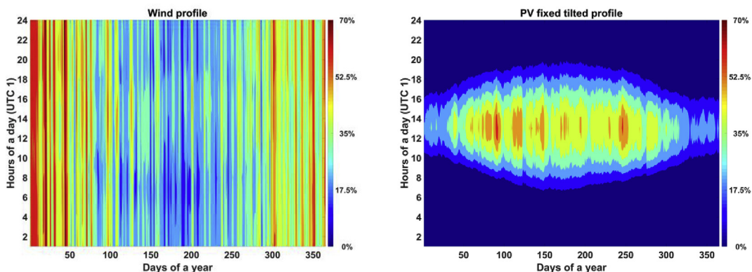
Fig. 15. Wind energy and solar PV generation profiles for the Area scenario in 2050.
