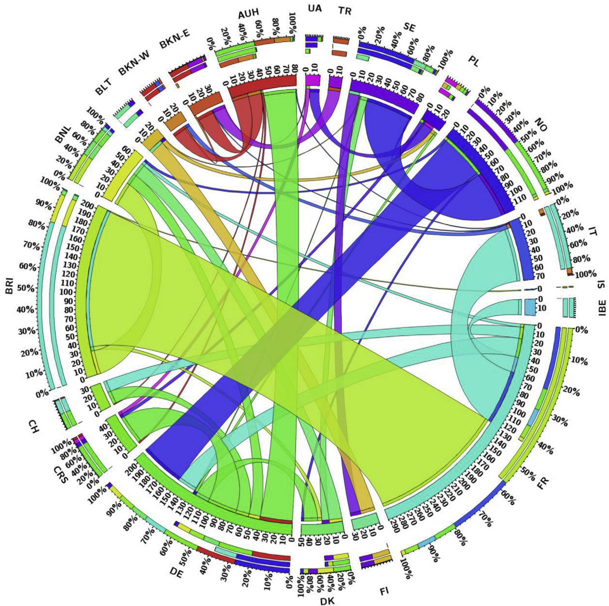
Fig. 18. Grid exchange between the regions of Europe for the Area scenario in 2050. Outer bars show relative exports, imports and overall totals for each region (from inside to out). Inner bars show absolute values of transmitted electricity for each colour-coded region (TWh). Central ribbons show the electricity exchanged from one region to another. Ends of the central ribbons indicate colour-coded regions of origin on one side, and regions of destination on the other. (For interpretation of the references to colour in this figure legend, the reader is referred to the Web version of this article.)
