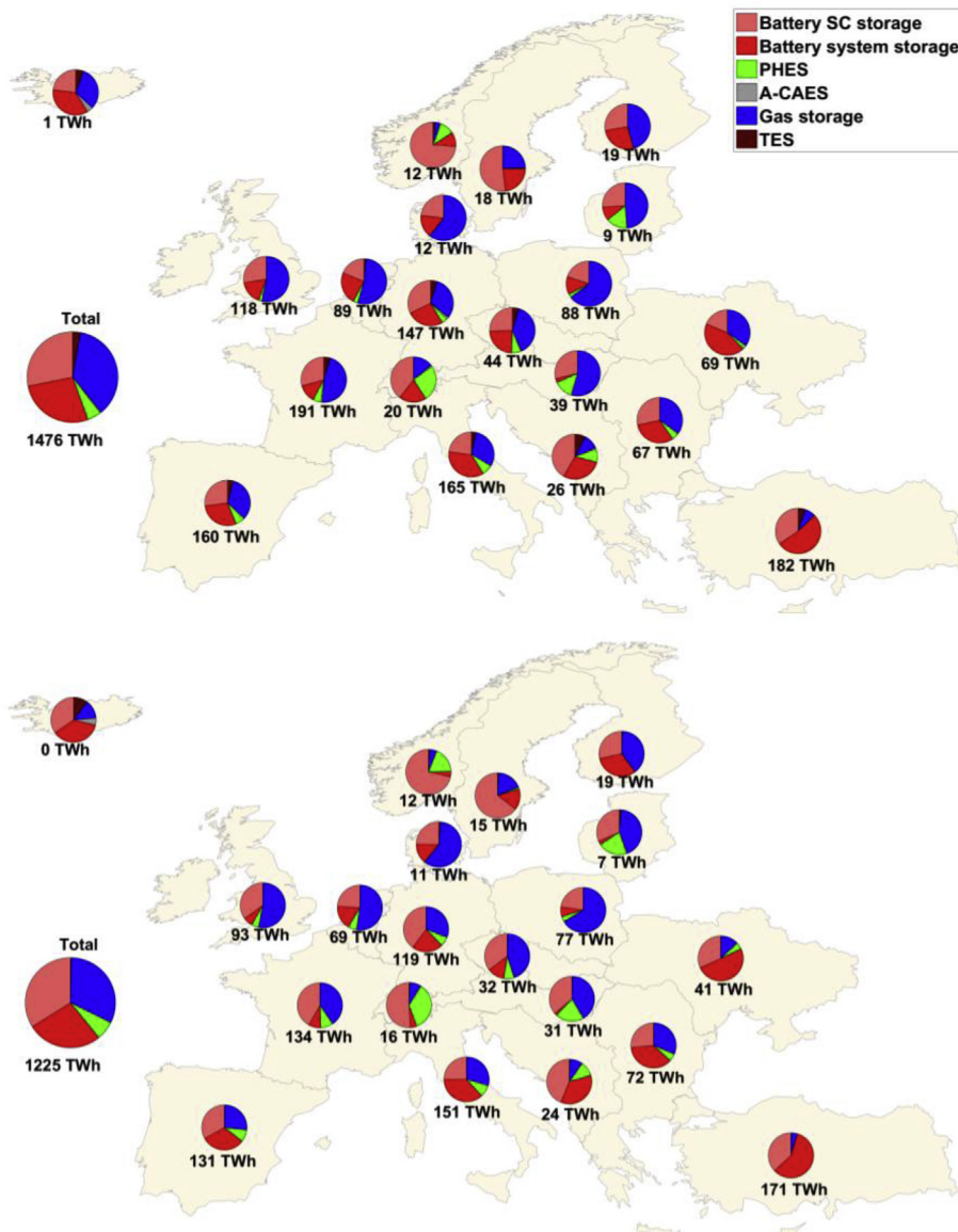
Fig. 11. Storage output for the Regions (upper) and Area (lower) scenarios for 2050. In this instance, output from storage is the sum of electrical, thermal and gas units to determine total storage output. Also, gas storage output includes dispatchable biomethane, in contrast to Fig. 10. Adapted from Ref. [39].
