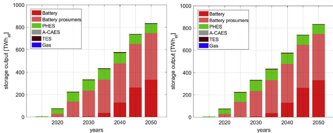
Fig. 10. Annual storage output of all technologies from 2015 to 2050 for the Regions (left) and Area (right) scenarios. Gas storage outputs do not include fossil natural gas or biomethane.
