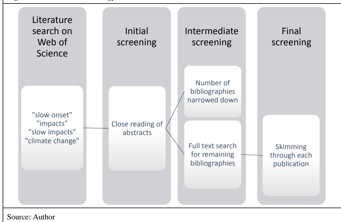
Figure 4: Review methodology
