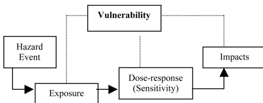
Figure 2: Risk-Hazard Model
