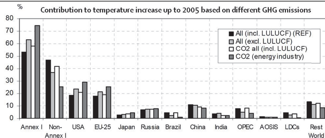
Figure 3: Relative contribution to temperature increase based on 1900–2005 emissions of all gases, including and excluding LULUCF and non-CO 2 gases for selected countries and country groups
