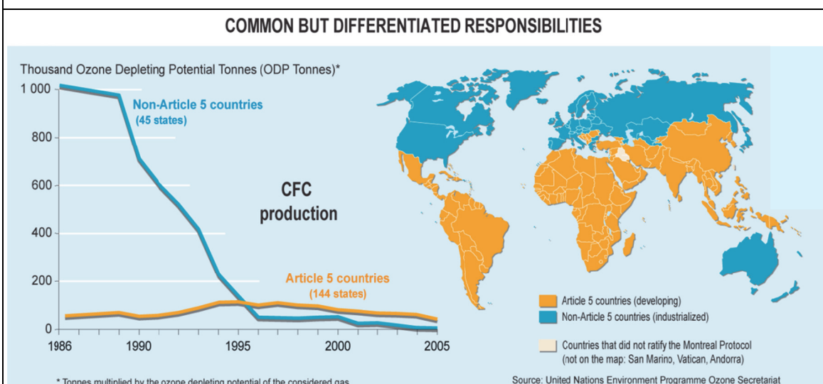
Figure 6: Emission of ozone-depleting substances by Article 5 and Non-Article 5 countries
