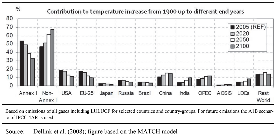
Figure 5: Relative contribution to temperature change from 1900 up to four different end years
