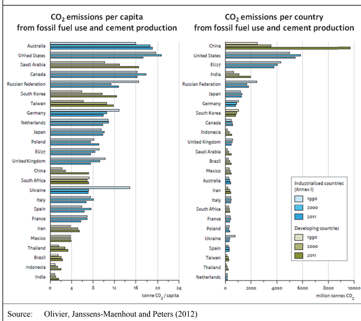
Figure 2: Global CO 2 emissions from fossil fuels and cement production: per capita / per country
