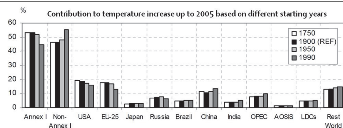
Figure 4: Relative contribution to temperature increase from four different starting years up to 2005
