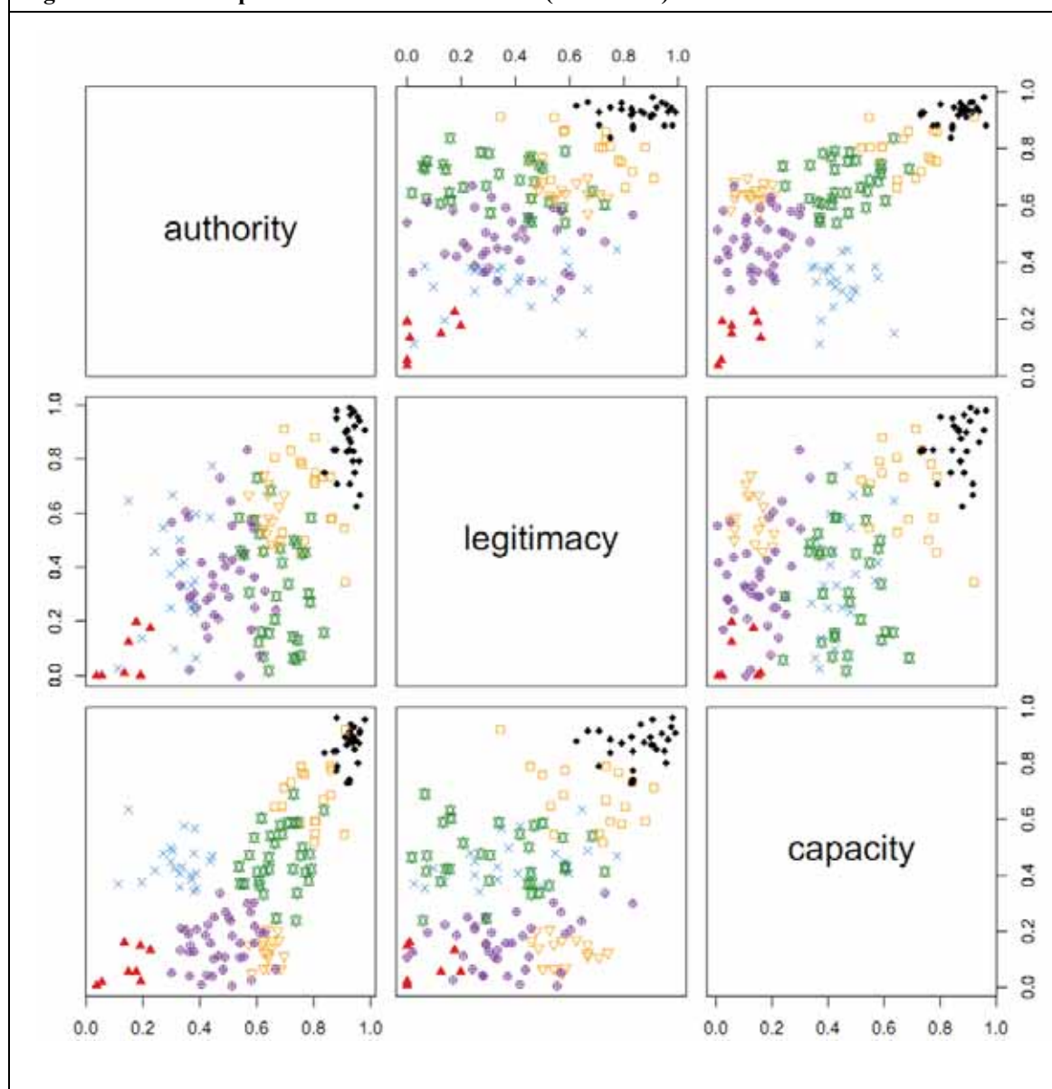
Figure 3: Scatter plots of the latent dimensions (2007–2009)
