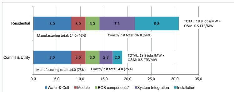
Figure 8: PV jobs per MW by value chain component (FTE-Year)
