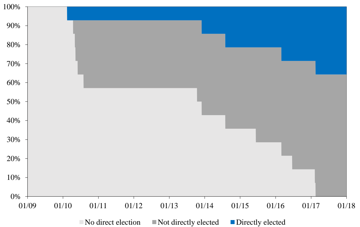
Figure 3: Sample balancedness
