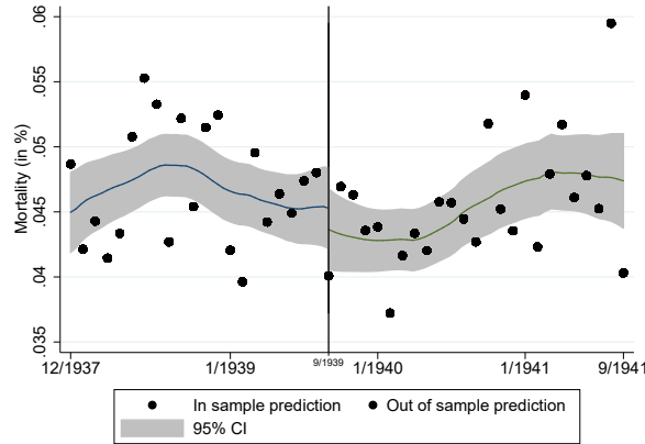
Figure 9: Predicted mortality
