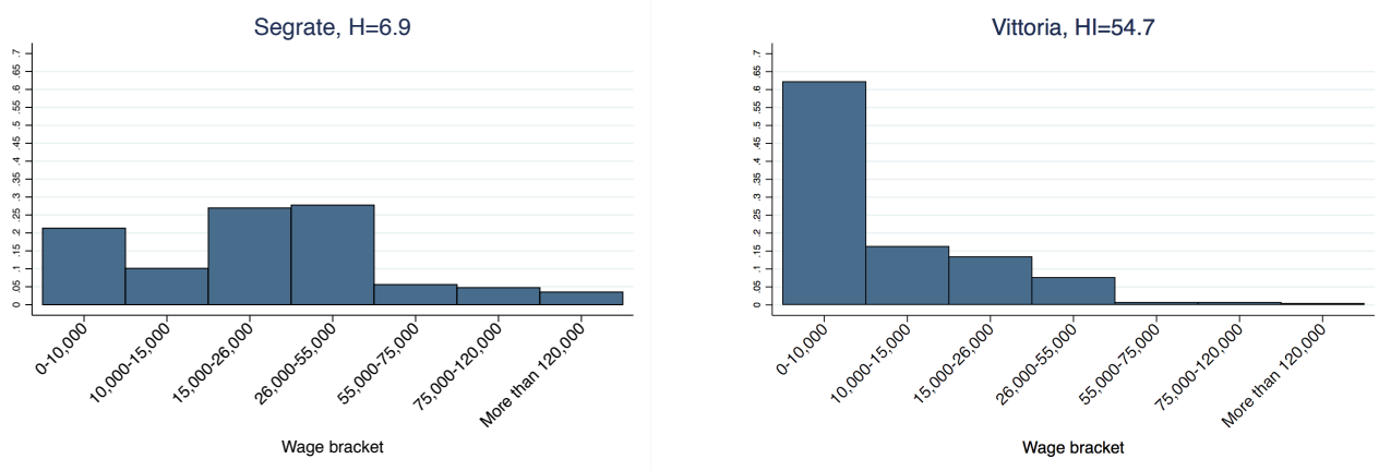
Figure 13: Left panels shows a municipality with uniform income distribution ( low concentration ), right panel shows a municipality with dispersed income distribution ( high concentration ).
