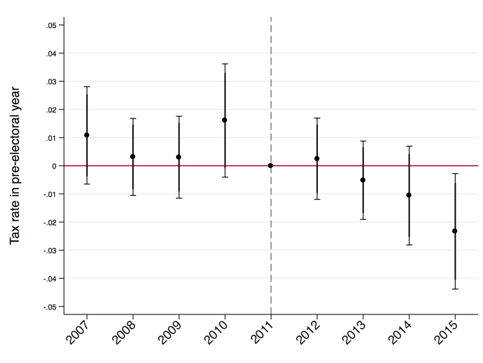
Figure 10: Pre-trends in terms of the median tax rate in the pre-election year.
