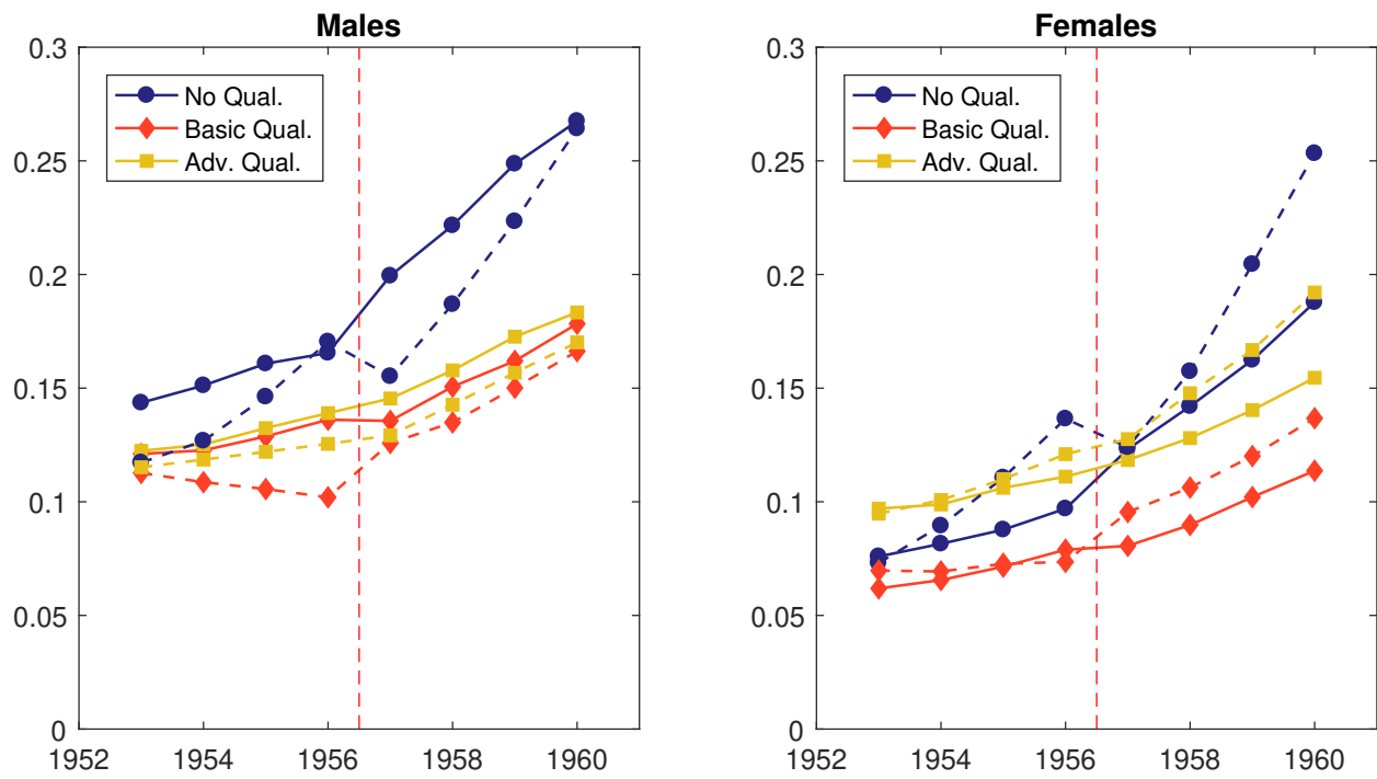
Figure D.1: Model Predicted (Constrained Model) and Empirical Never-Married Rates by Cohort, Gender, and Qualification Level
