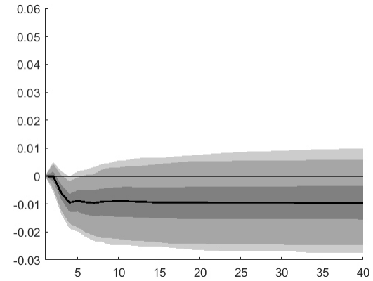
Figure 19. Figure 19a and 19b report the response (in levels) of US TFP following a one standard deviation innovation in a model controlling for asset returns, and when an alternative news factor is used, respectively. The black solid line is the median estimate. The uncertainty bands reflect the 95, 90, and 50 percent quantiles, constructed from a residual bootstrap.
