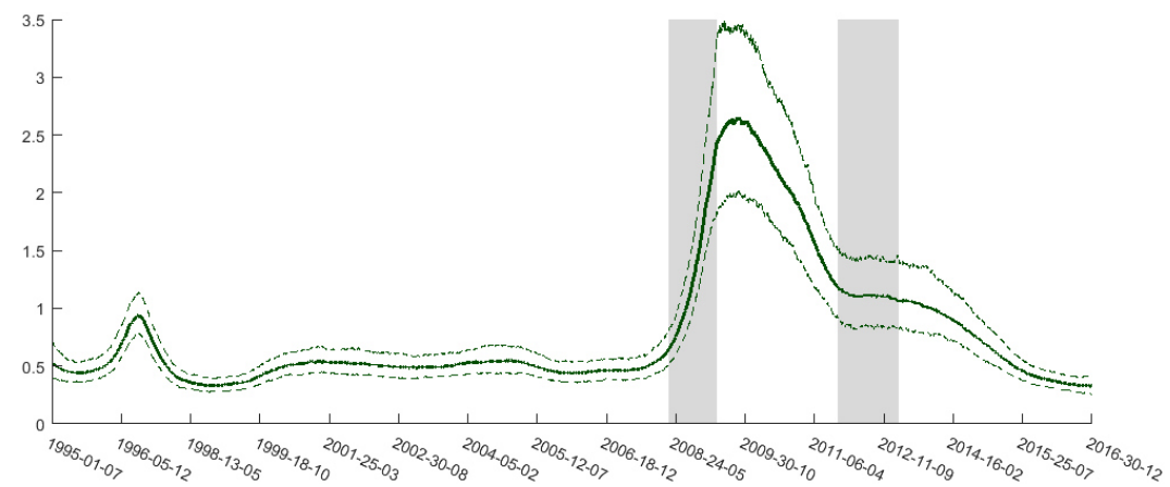
Figure 10. Standard error of the stochastic error in the daily coincident indexes. The colored solid line is the median, while the colored dotted lines are the 68 percent probability bands. The gray shaded areas illustrate recession periods as defined by NBER (US), ERCI (Japan), and CEPR (euro area).
