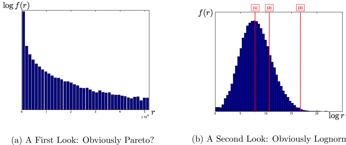
Figure 15: Alternative Perspectives on the Data
