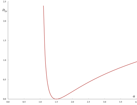
Figure 12: KLD as a Function of \sigma in the Pareto-CREMR Case
