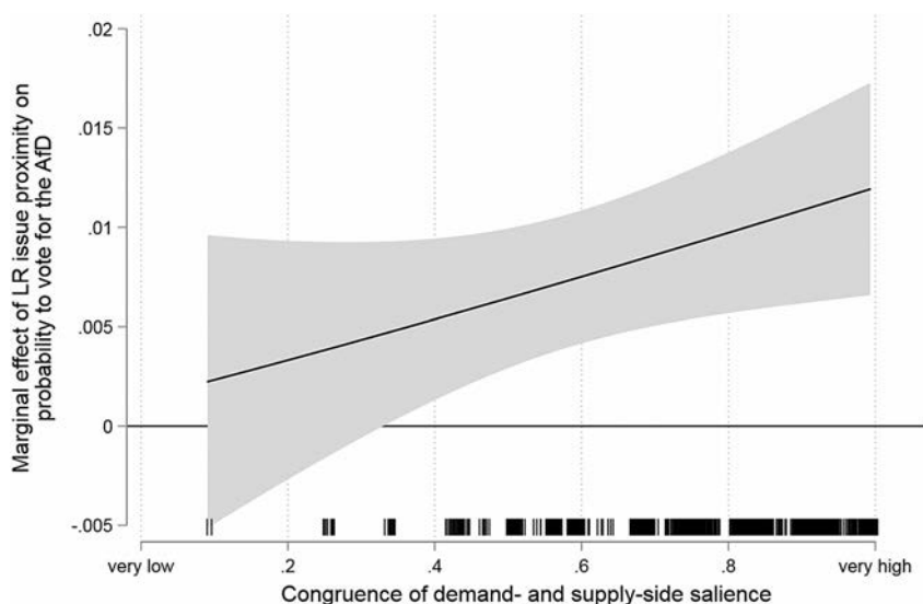
Figure 4. Conditioning effect of salience congruence on left-right proximity for AfD vote intention.
