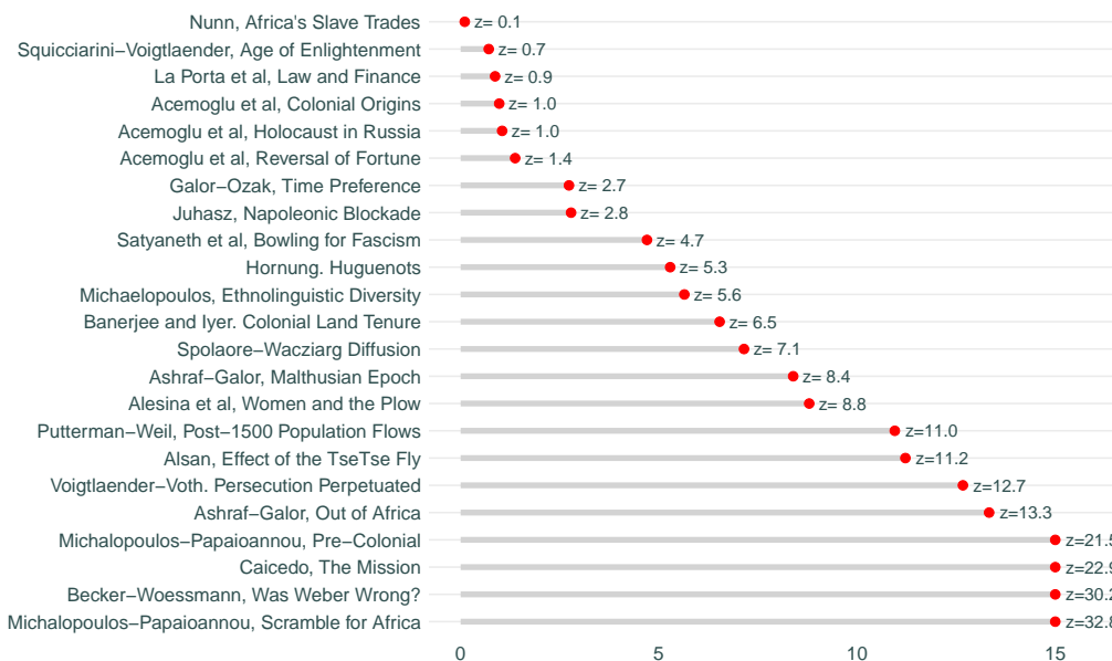
Figure 7: Z scores of Moran tests for spatial autocorrelation in regression residuals.
