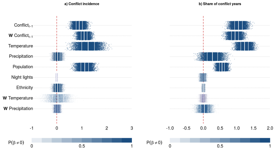
Figure 6: Local conflict determinants for conflict incidence (a) and the share of conflict years between 2003-2017 (b). Each blue point in the plot represent a draw from the posterior distribution for the respective variable coefficient; with vertical lines indicate the mean and 66% uncertainty interval. The posterior inclusion probability of a variable is reflected by the opacity of the points with full transparency indicating P(\beta \neq 0|y, X) = 0 and full opacity indicating P(\beta \neq 0|y, X) = 1 .
