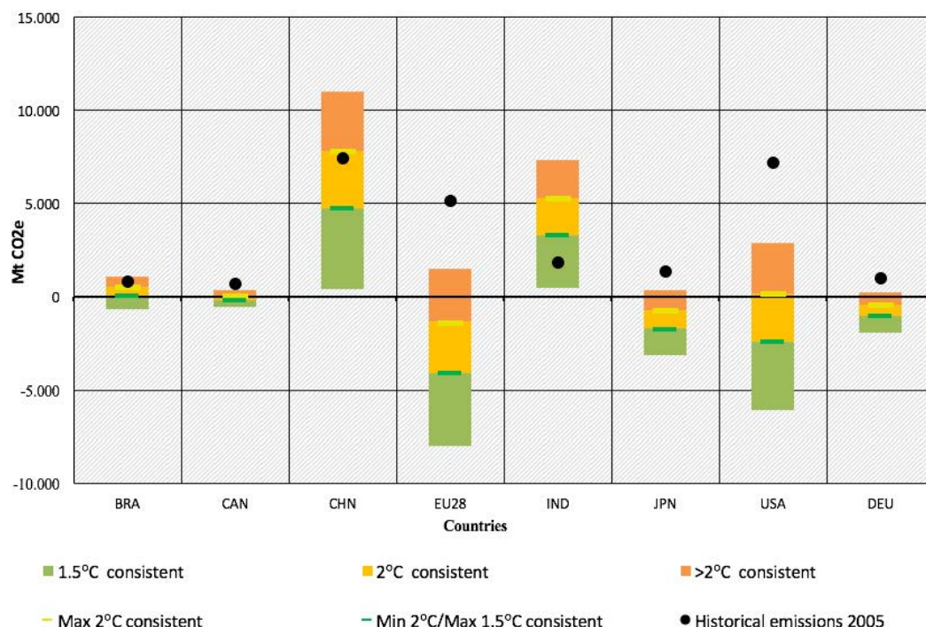
Figure 4: Effort sharing range of total GHG emissions in 2050
