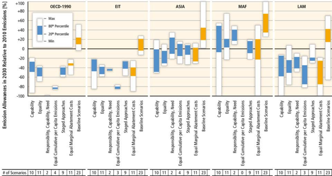
Figure 1: Emissions allocation in 2030 relative to 2010 emissions by effort sharing category for 2°C compatible mitigation scenarios (reaching 430 – 480 ppm CO 2 eq. in 2100).
