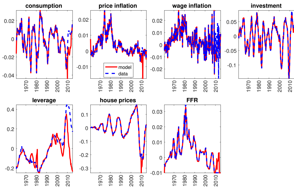
Figure A3: Smoothed Variables and Data
