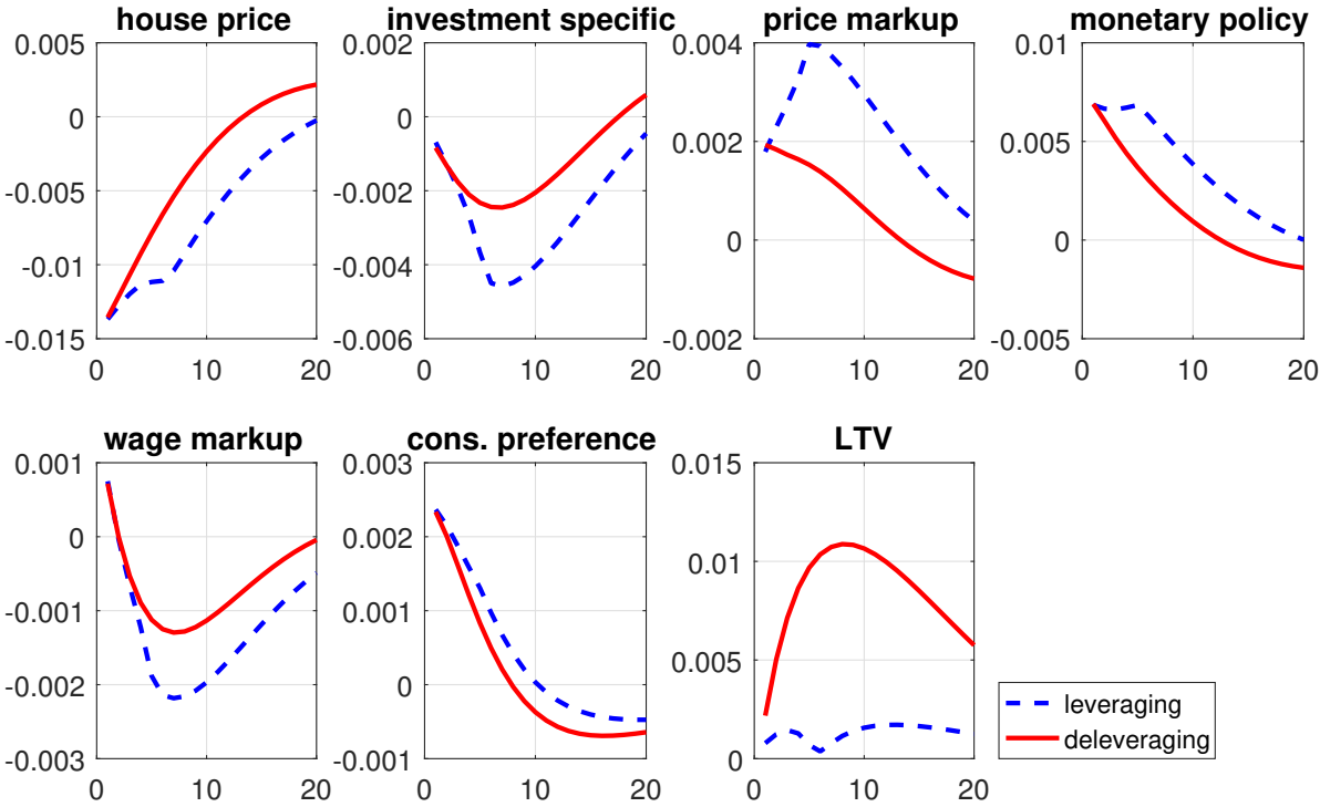
Figure A5: IRFs of Leverage to all Shocks during Leveraging and Deleveraging
