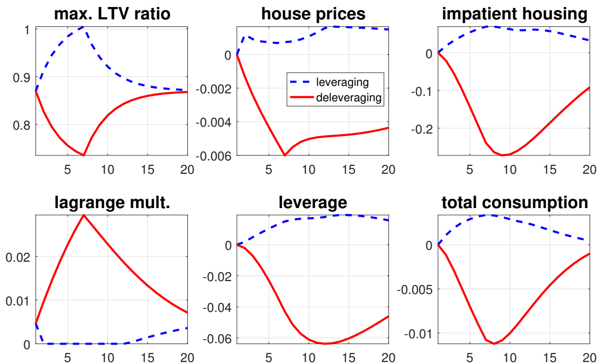
Figure 6: Sequence of Positive and Negative LTV Shocks
