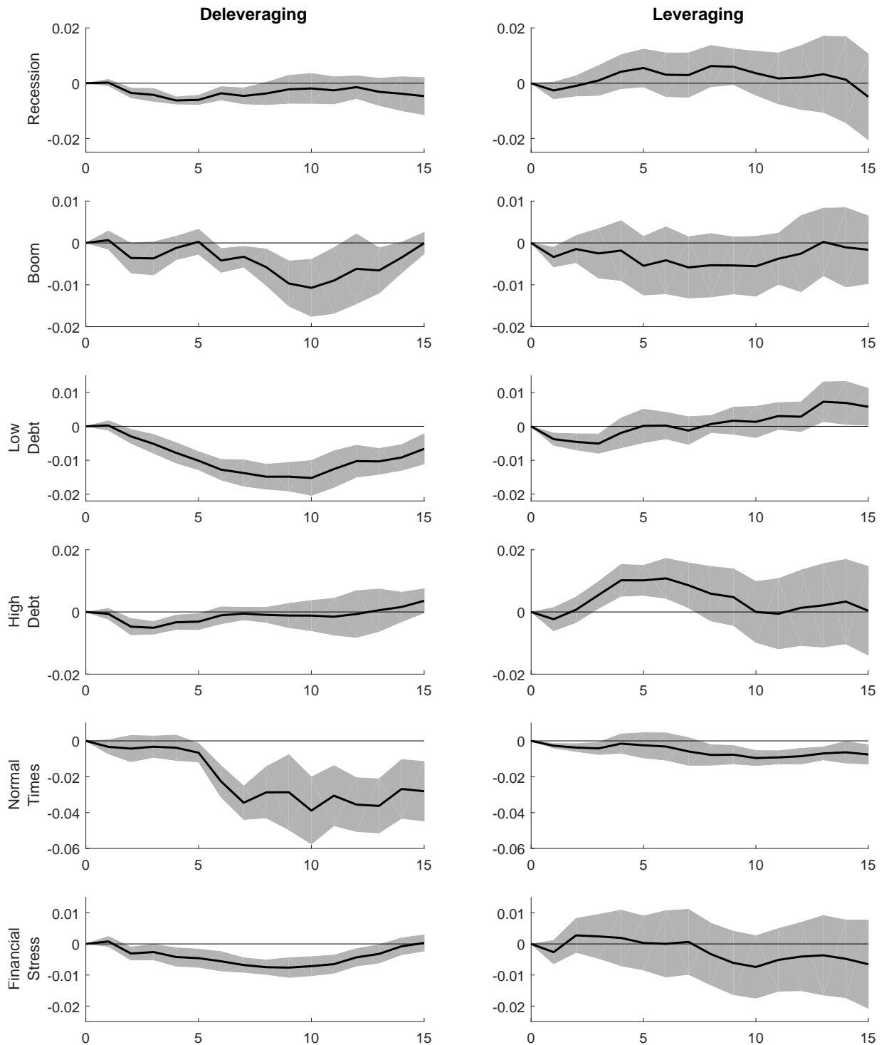
Figure 5: Controlling for Additional States (GDP responses)
