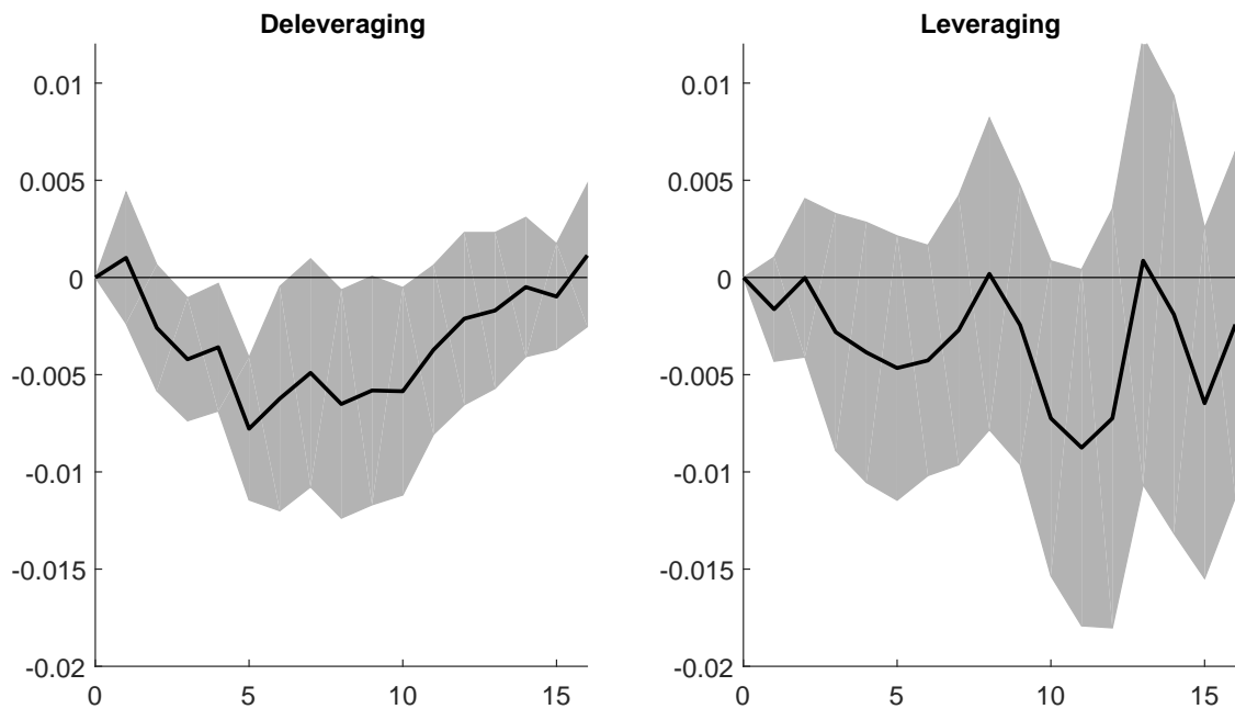
Figure A1: Nonlinear Romer and Romer (2004) Shocks (GDP responses)
