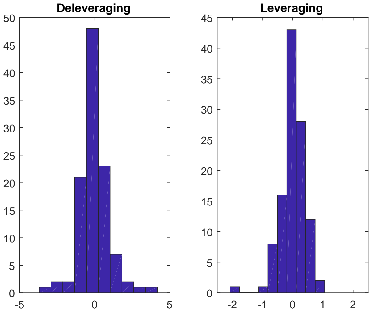
Figure A2: Distribution of Monetary Policy Shocks
