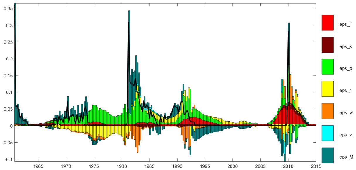
Figure 12: Shock Decomposition: Nonlinear Model
