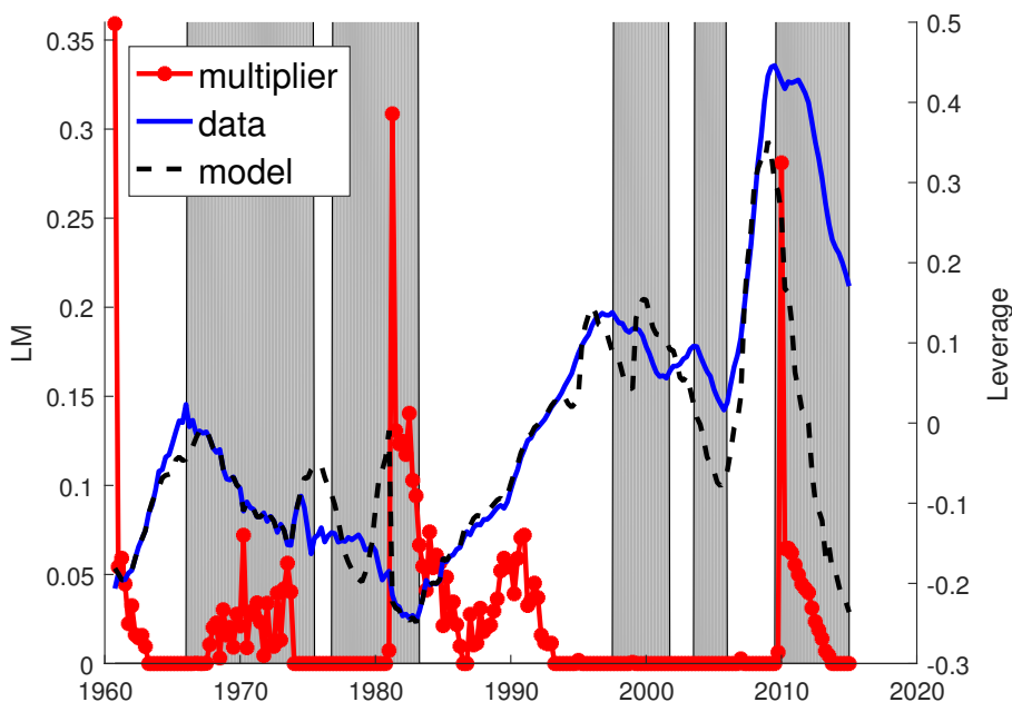
Figure 8: Deleveraging and Borrowing Constraints
