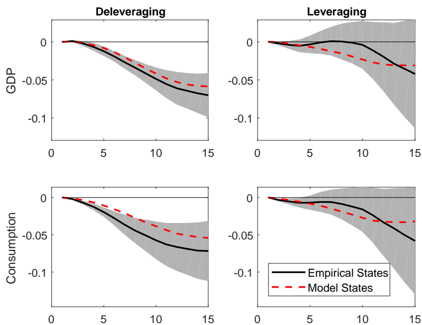
Figure 9: Cumulative Effects: Empirical States and Model States
