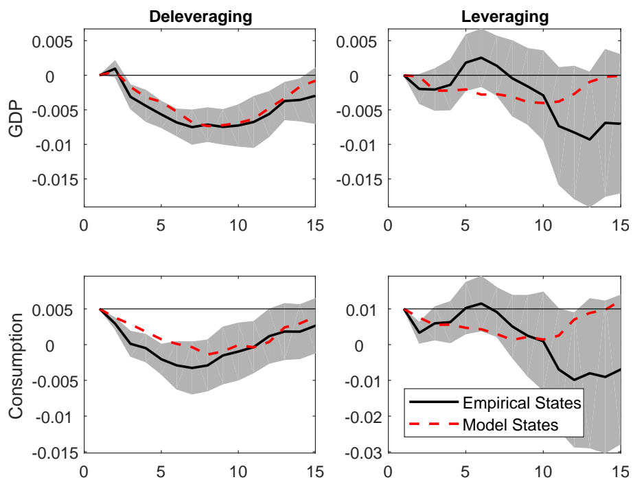
Figure A4: Non-Cumulative Effects: Empirical States and Model States
