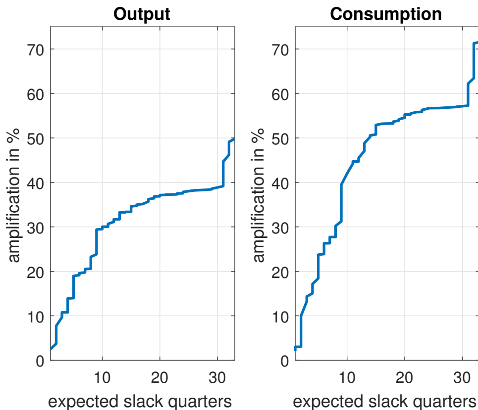
Figure 11: Amplification Effects After a Monetary Policy Shock
