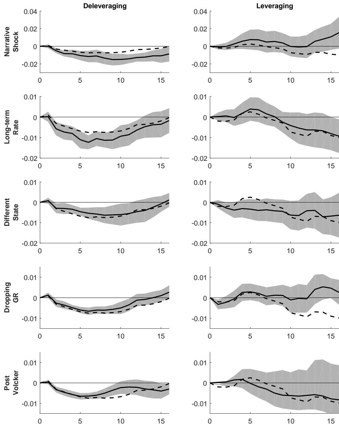
Figure 4: Robustness (GDP responses)
