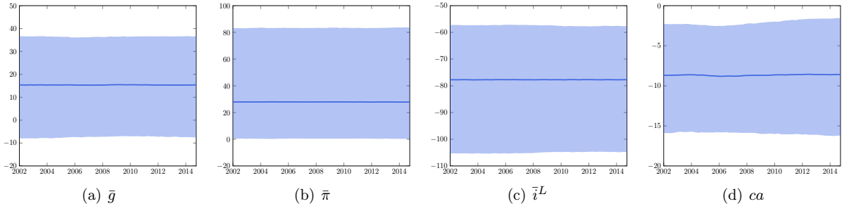
Figure 3: Structural parameters \beta_{kt}
