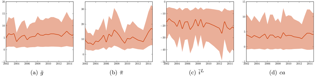
Figure 4: Expectations of parameters E_t(\beta_{kt})
