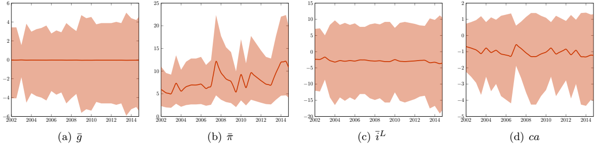
Figure 4: Expectations of parameters E_t(\beta_{kt}) (cont'd)
