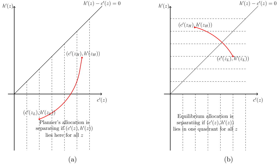
Figure 2: Assume (7) is satisfied. In (a), h is not monotone in z , so the equilibrium will involve some pooling. However, since h'(\cdot) - c'(\cdot) \leq 0 , the planner achieves the first best through a separating allocation (Proposition 3(iii)). In (b), equilibrium is separating because h'(\cdot) \geq 0 . However, h - c is not decreasing, so the planner cannot achieve the first best and the constrained efficient allocation may not be separating.
