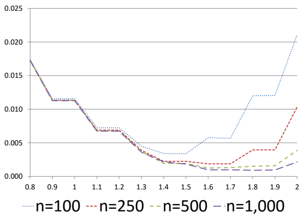
(c) V_0 \sim N(0, 1)
