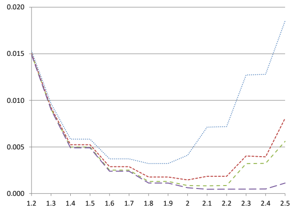
(b) V_0 \sim N(0, 0.5)
