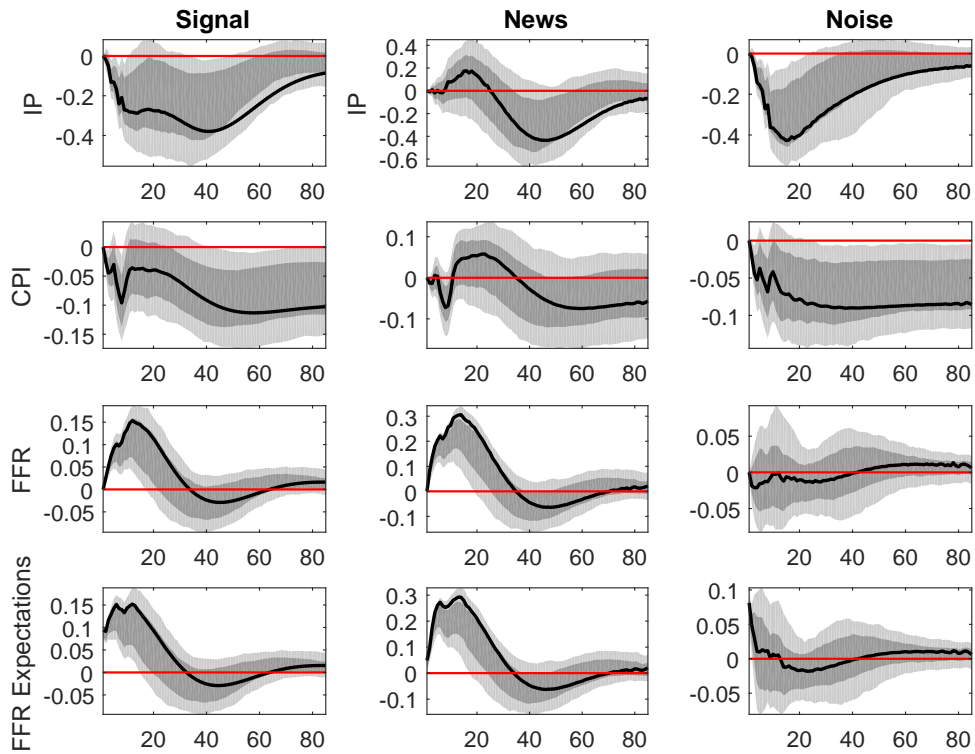
Figure 3: Four-variate VAR: Signal, News, and Noise
