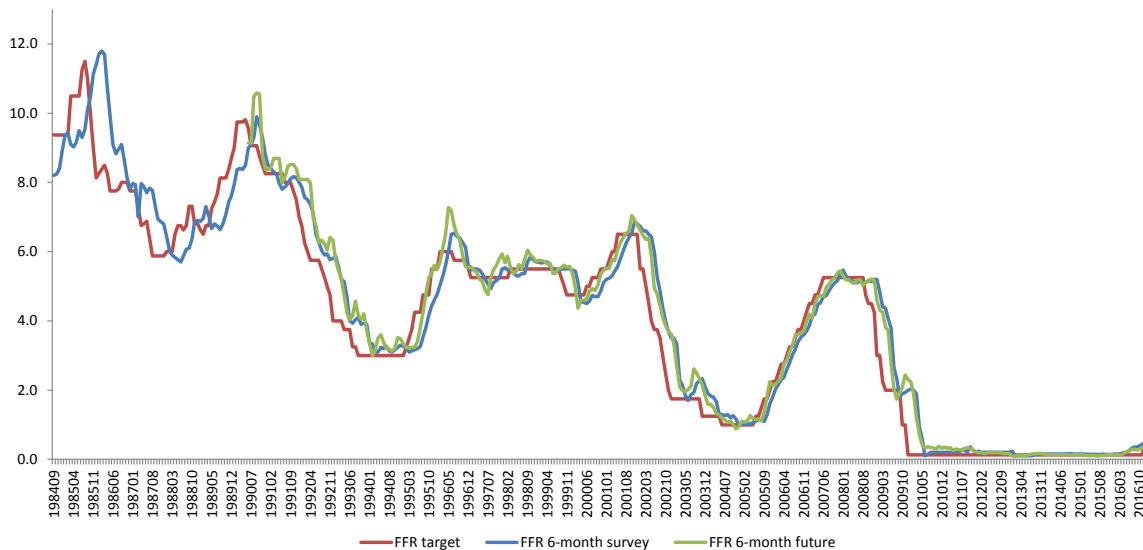
Figure 1: Fed Funds Rate and its Expectations
