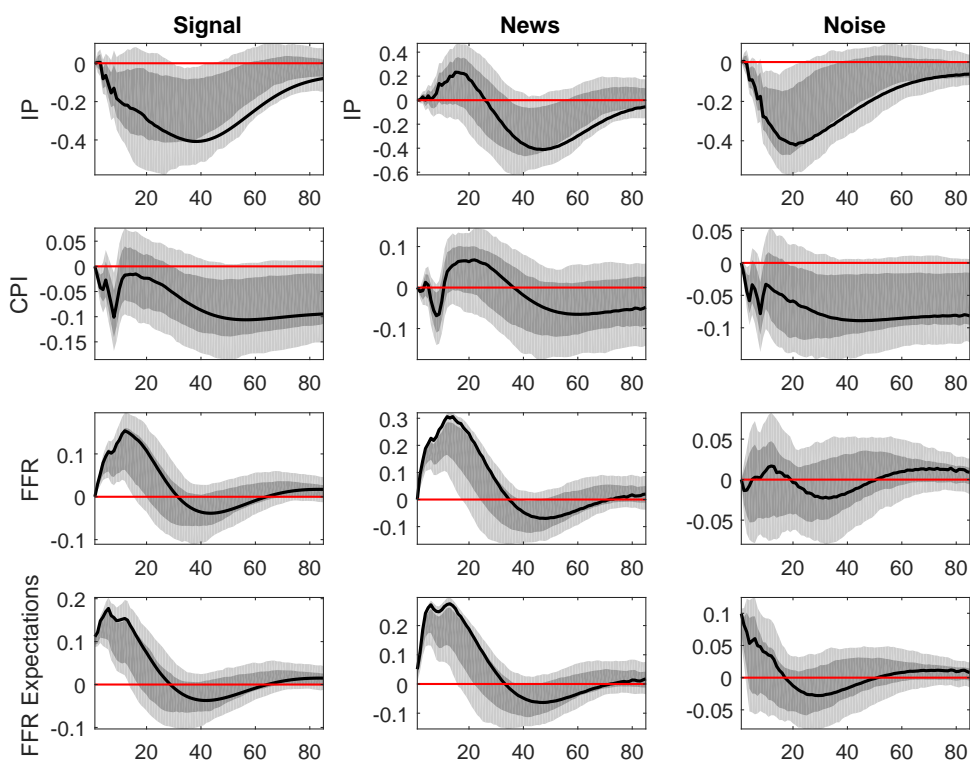
Figure 4: Four-variate VAR (Incl. Nine-month Expectations): Signal, News, and Noise
