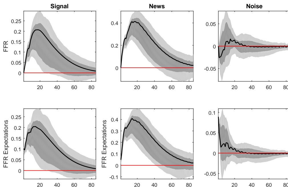
Figure 2: Bivariate VAR: Signal, News, and Noise
