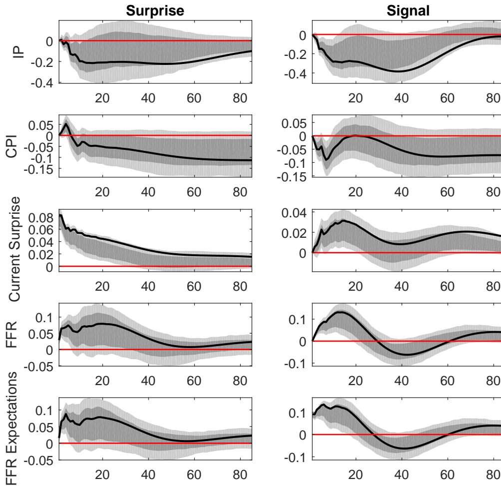
Figure 8: Five-variate VAR with Conventional Monetary Policy Shock: Surprise and Signal
