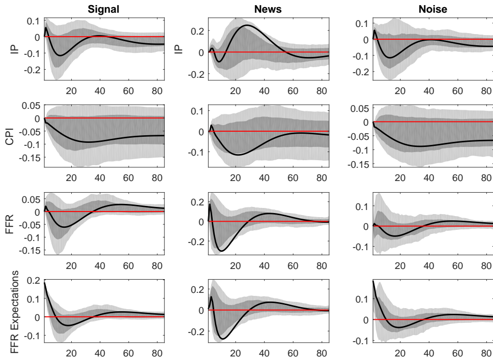
Figure 6: Four-variate VAR before 1994: Signal, News, and Noise
