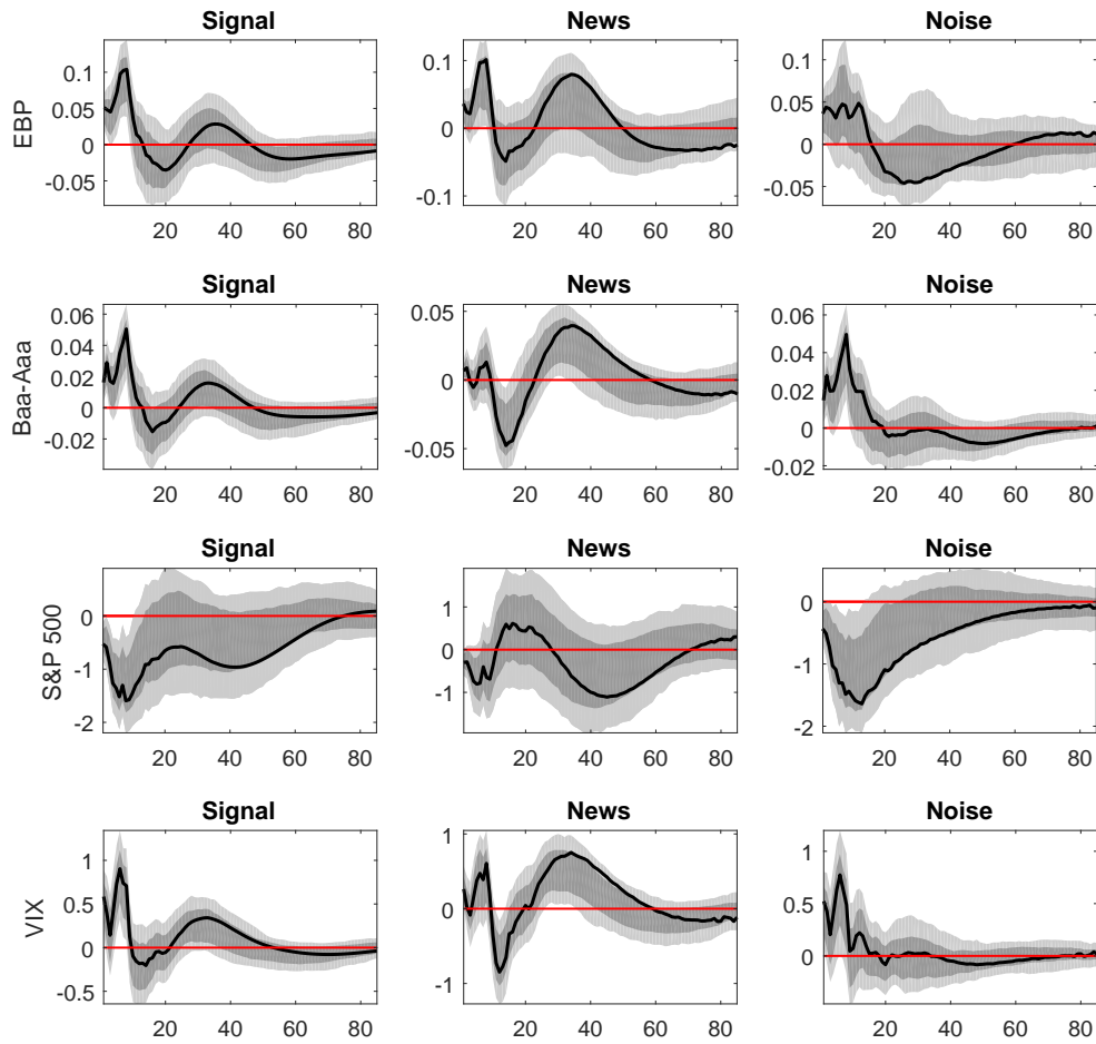
Figure 7: Five-variate VARs with Financial Indicators: Signal, News, and Noise
