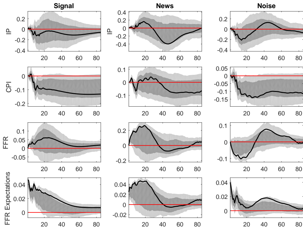
Figure 5: Four-variate VAR (Incl. Market-based Expectations): Signal, News, and Noise
