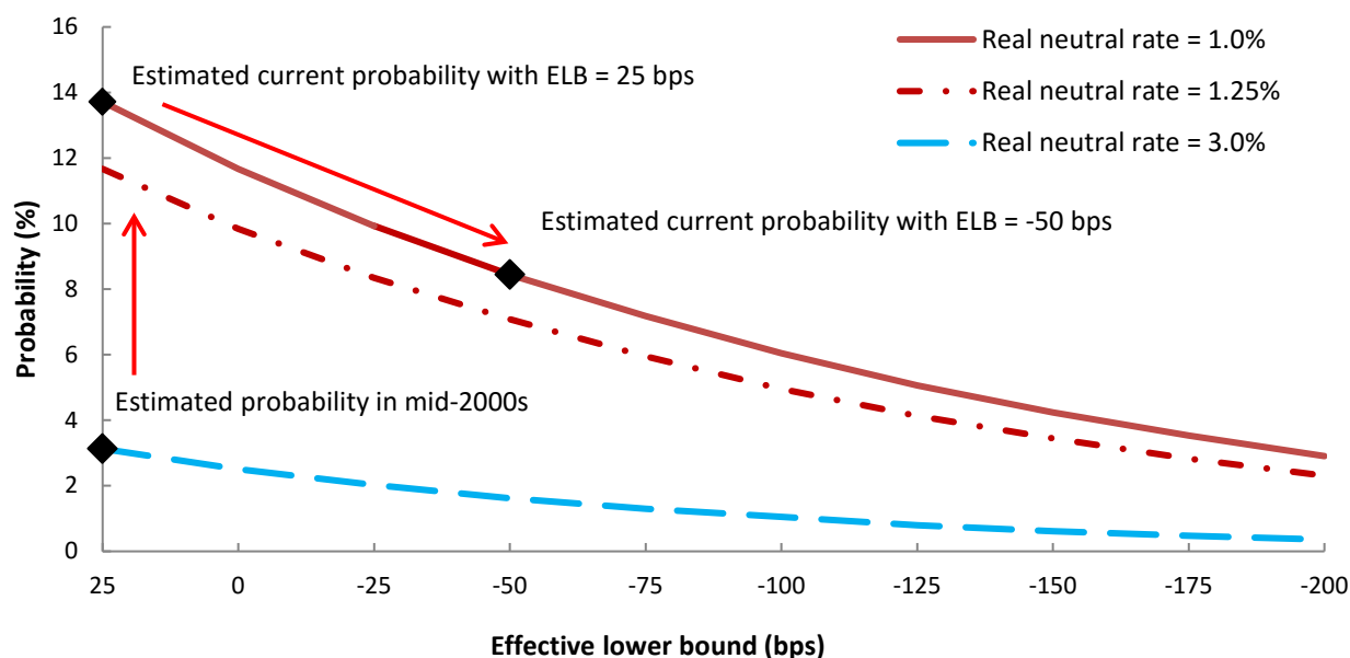
Figure C.1: Unconditional probability of binding ELB constraint for different neutral rates
