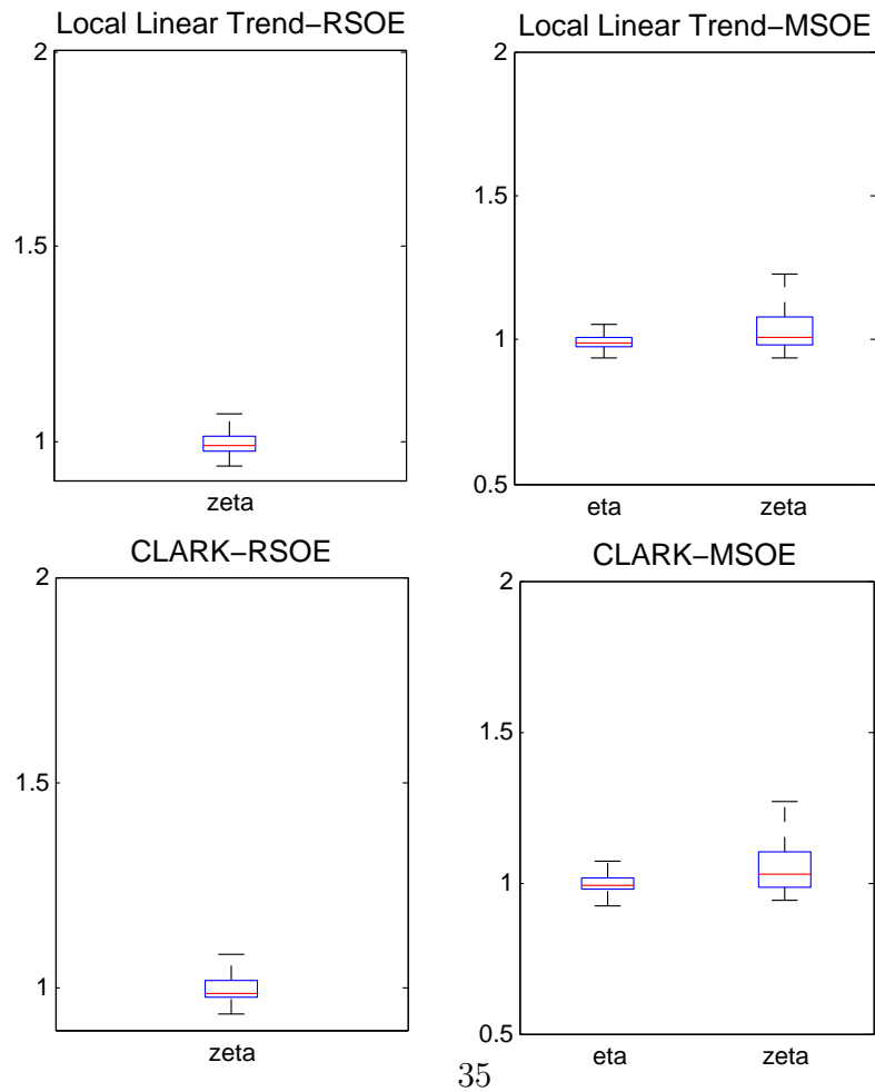
Figure 6: Inefficiency Factors for Disturbance Smoothing (I(2)-UC Models)
