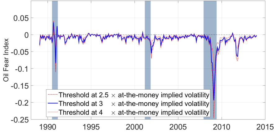
Figure 1: Oil market fear index, FI_t \equiv RJV_{t,T}^{\mathbb{Q}} - LJ V_{t,T}^{\mathbb{Q}} , in annualized form. Different lines stand for different thresholds for the definition of large jumps in the computation of FI_t . Shaded areas represent NBER recessions. The sample period is 1989:1 to 2013:12.
