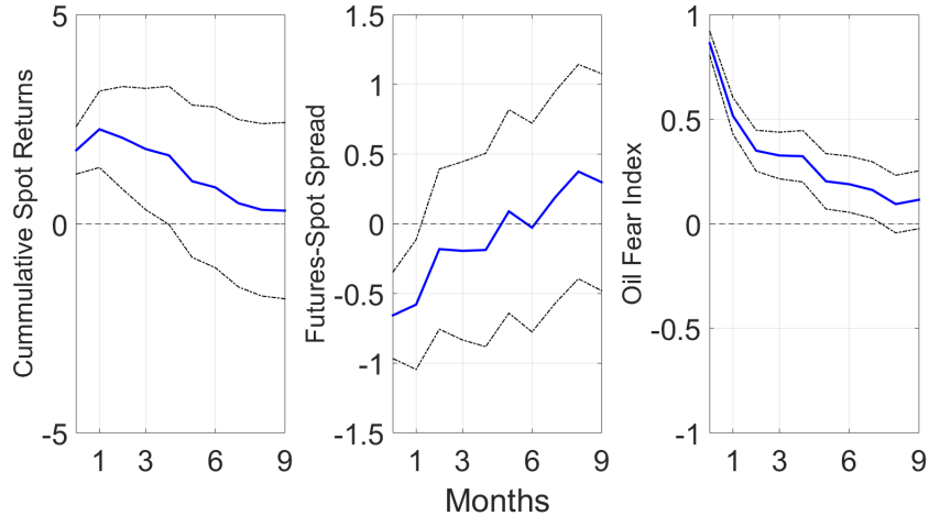
Figure 3: Responses of the spot price of oil, the 12-month futures spread and the oil market fear index to a one-standard-deviation shock in the oil market fear index, FI_t . The estimates are based on a Cholesky decomposition with the following order: oil production, real economic activity, change in inventories, FI_t , futures spread, and oil spot returns (left and right panel); oil production, real economic activity, change in inventories, FI_t , futures spread, and oil spot (middle panel). Dashed lines represent 90% asymptotic confidence intervals. The sample period is 1989:1 to 2013:12.
