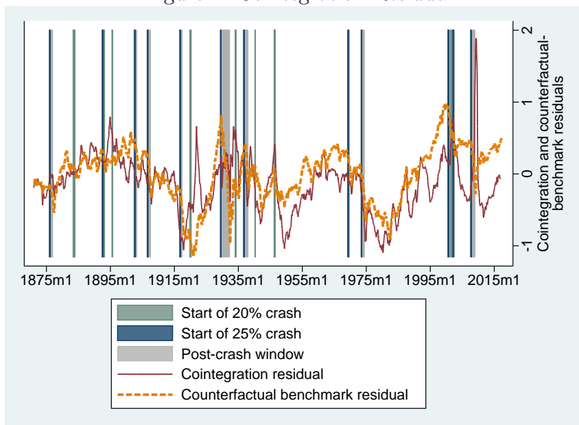
Figure 2: Cointegration Residual
