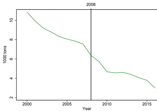
(e) PM10 emissions in Western EU
