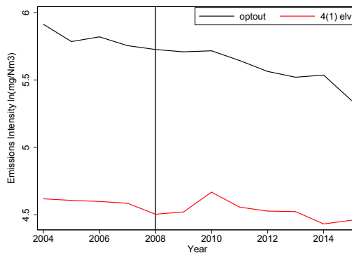
(b) NOx - Opt Out MS
