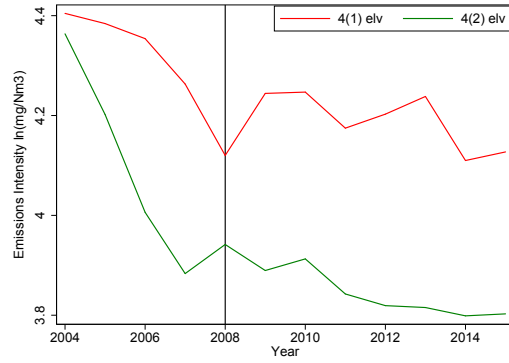
(b) NO x - Affected by IPPC
