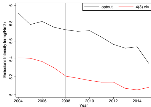
(a) NOx - Opt Out MS
