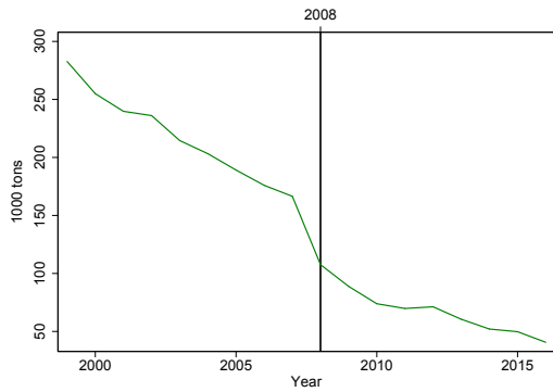
(c) SO2 emissions in Western EU
