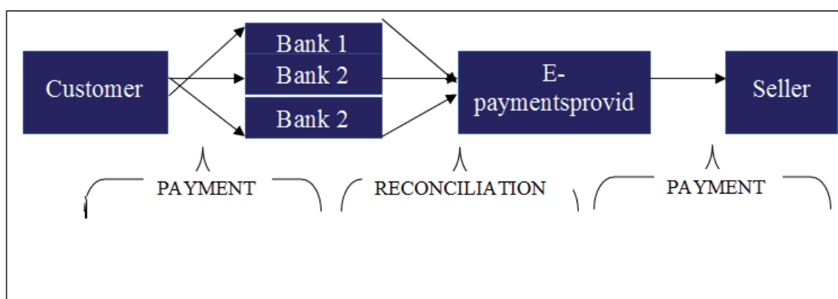
Figure 1: E-payment model
