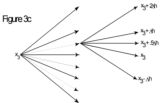
Figure 3: Construction of the lattice
