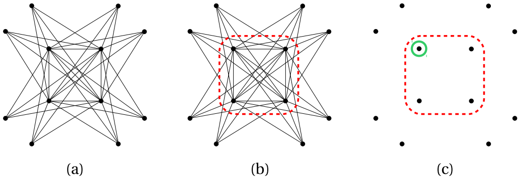
FIGURE 13. Separators and transversals in interlinked stars ( n = 12 ).
