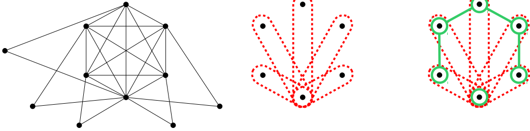
FIGURE 8. Network with essential separators of size 2 having two minimal transversals: one of size 1 and one of size 5.
