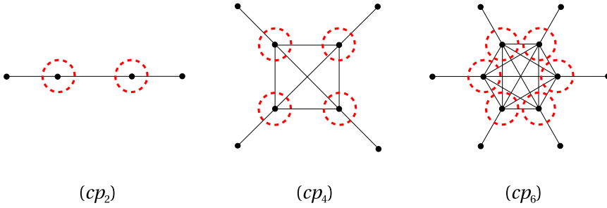
FIGURE 9. Core-periphery networks cp_2 , cp_4 , and cp_6 .
