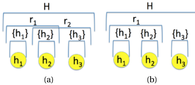
FIGURE 1. An example of sets of regions in Example 1. (a) A non-hierarchical set of regions R . (b) A hierarchical set of regions R' .
