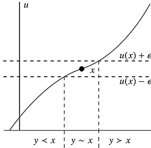
FIGURE 4. A semiorder representation.
