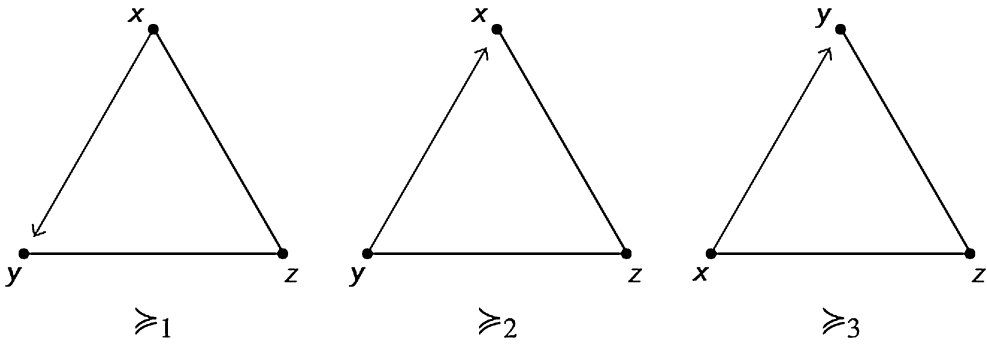
FIGURE 3. Illustration of Theorem 1.
