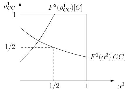
FIGURE 1. Beliefs equilibrium.
