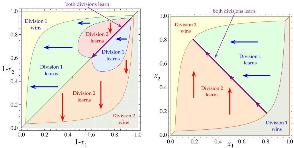
(a) D_1 and D_2 each operates the bad-news technology (BNT).
