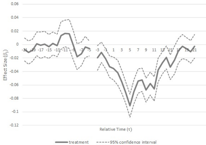
FIGURE 5 EVENT STUDY
