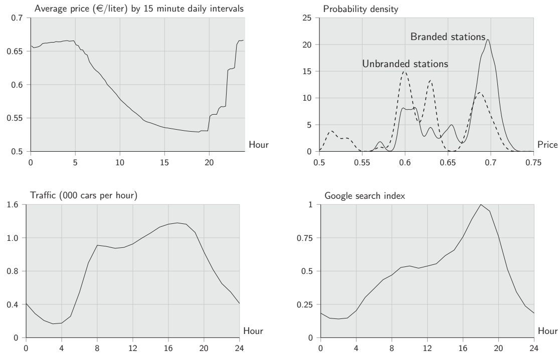
Figure 3 Data description
