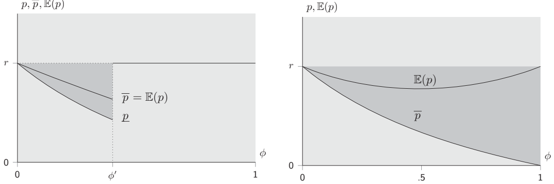
Figure 1 Proposition 1 illustrated
