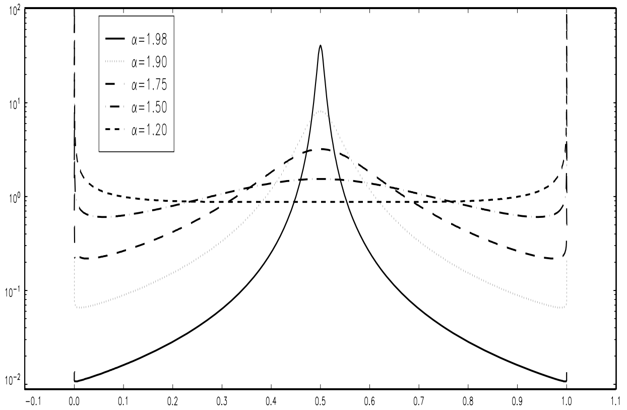
Figure 2. Probability density functions of \tilde{R}(\alpha, \eta)
