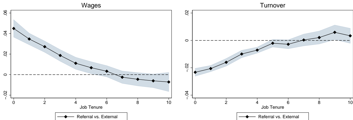
FIGURE 4: CONVERGENCE PROFILES
