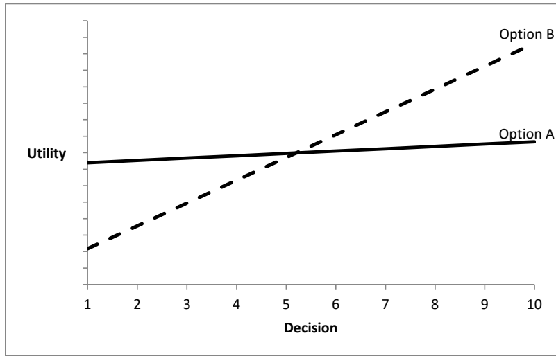
CLAPT : x = 0.2; \lambda = 2.2
