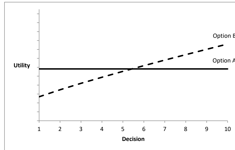
RDEU : x = 0.3; \alpha = 0.85
