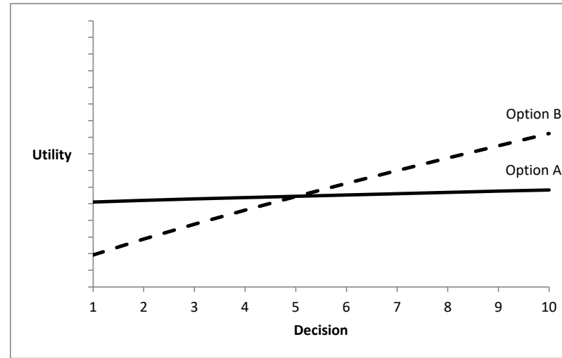
RDEU : x = 0.3; \alpha = 0.85
