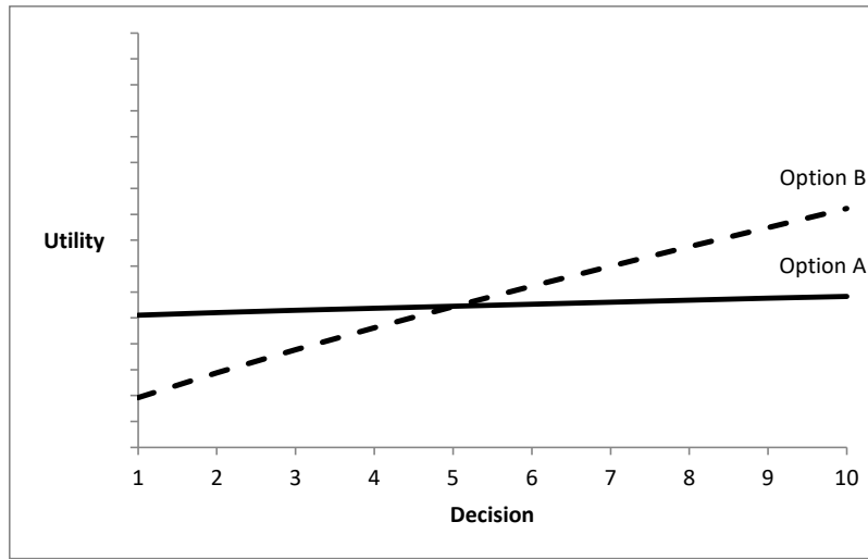
PWPT : x = 0.3; \alpha = 0.85; \beta = 0.25
