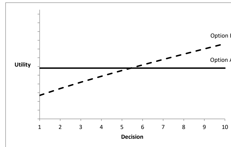
PWPT : x = 0.3; \alpha = 0.85; \beta = 0.25
