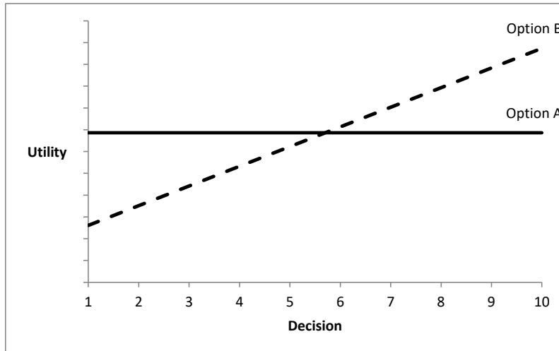
CLAPT : x = 0.2; \lambda = 2.2
