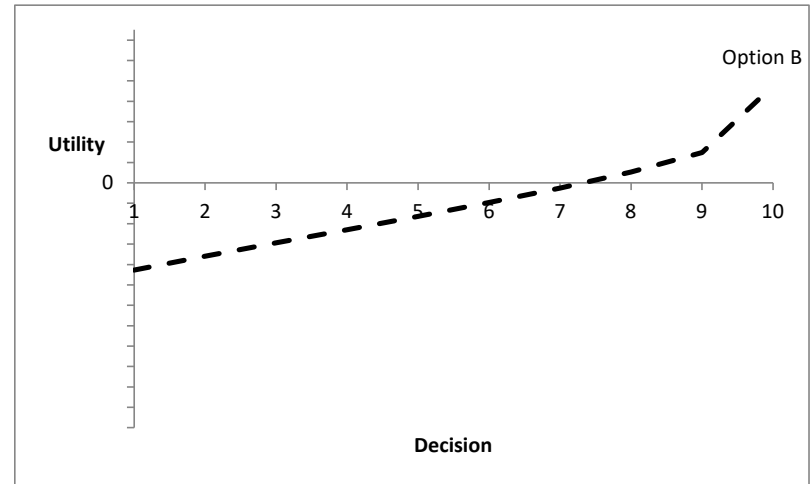
PWPT : x = 0.3 ; \alpha = 0.85 ; \beta = 0.25
