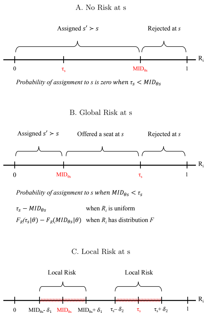
Figure 2: Visualizing Risk under Serial Dictatorship
