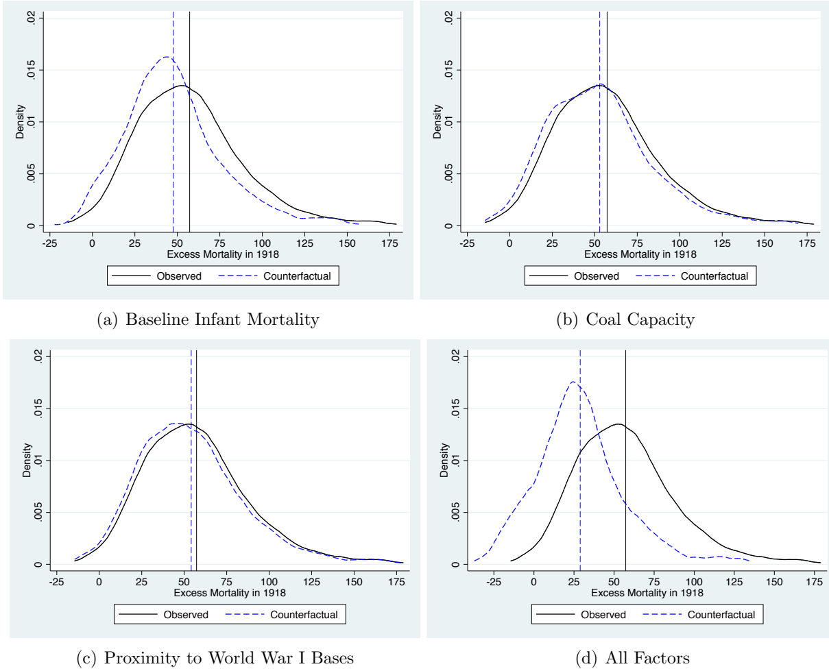
Figure 3: Excess Mortality and Counterfactual Excess Mortality in 1918
