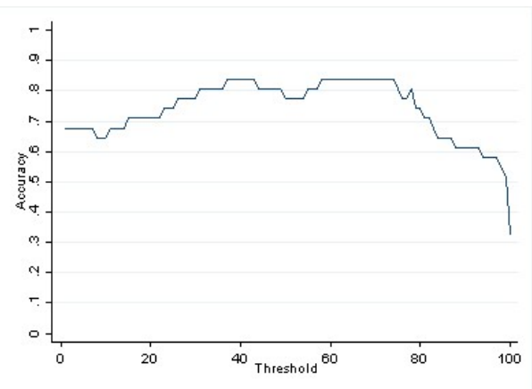
Figure 3. Accuracy rates of logit predictions depending on the classifying probability threshold in percent for STC.
