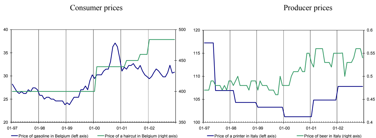
Figure 1 - Examples of individual price trajectories
