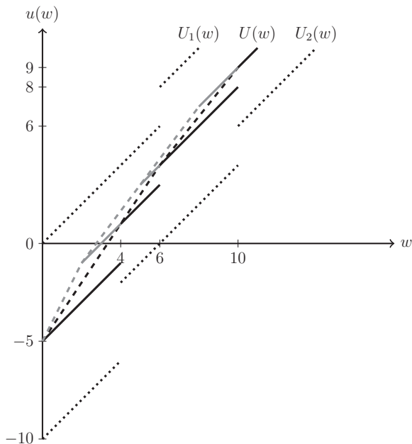
Figure 2: Example 2. The black dotted lines denote state-dependent utility U_s(w) . The black solid line denotes U(w) . The black dashed line denotes \bar{U}(w) . The gray solid line denotes U_I(w) if it exceeds U(w) . The gray dashed line denotes U^*(w) .
