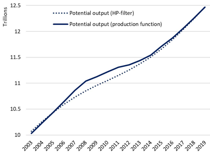
Figure 2: Potential output estimates using the production function method and the HP filter
